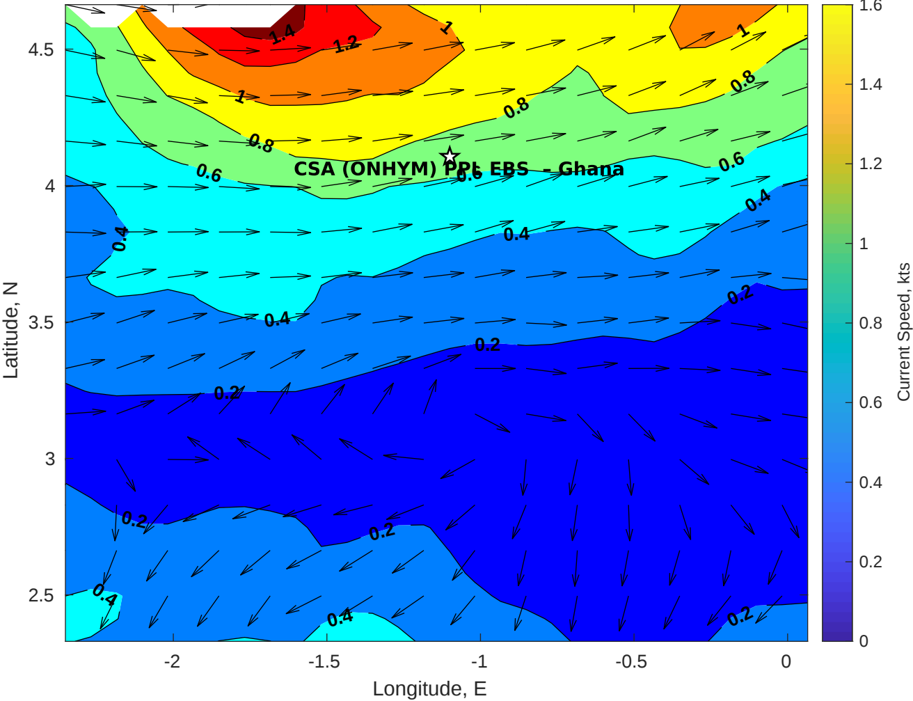
Surface Currents for CSA (ONHYM) PPL EBS - Ghana at 24-Nov-2025 00:00:00
