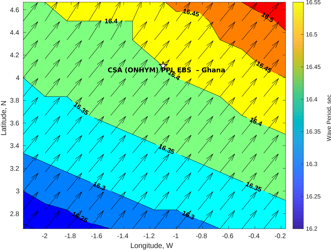
GFS Wave Period (sec) for CSA (ONHYM) PPL EBS - Ghana at 25-Nov-2025 09:00:00
