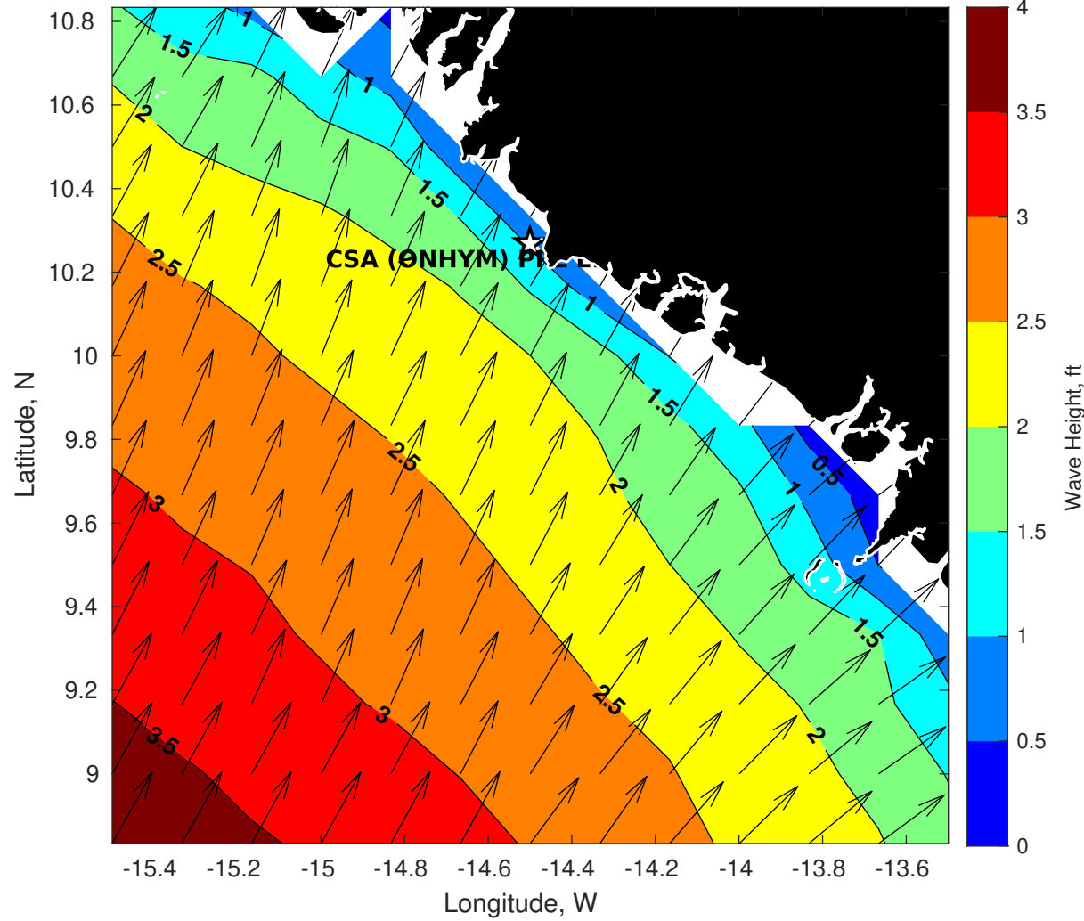
GFS Wave Height (ft) for CSA (ONHYM) PPL EBS - Guinea at 25-Nov-2025 09:00:00
