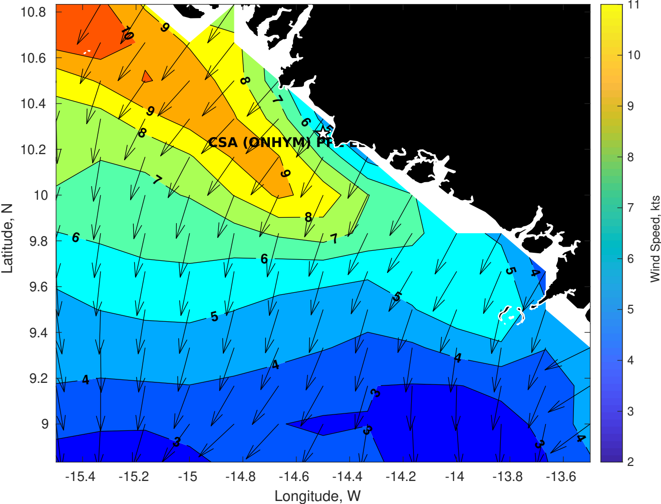
GFS Winds (kts) for CSA (ONHYM) PPL EBS - Guinea at 25-Nov-2025 09:00:00
