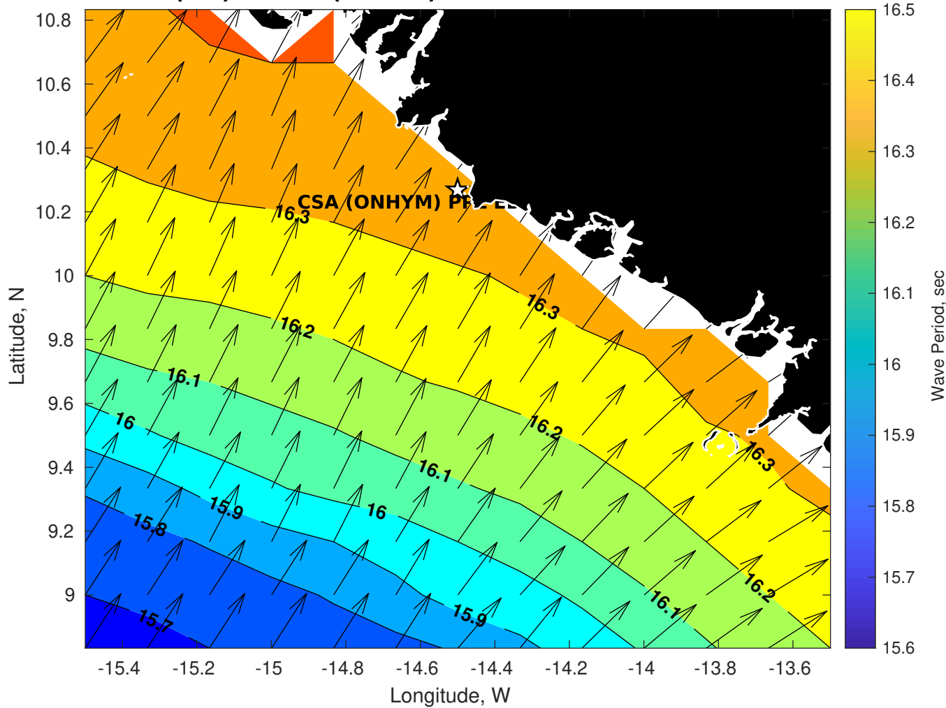
GFS Wave Period (sec) for CSA (ONHYM) PPL EBS - Guinea at 25-Nov-2025 09:00:00
