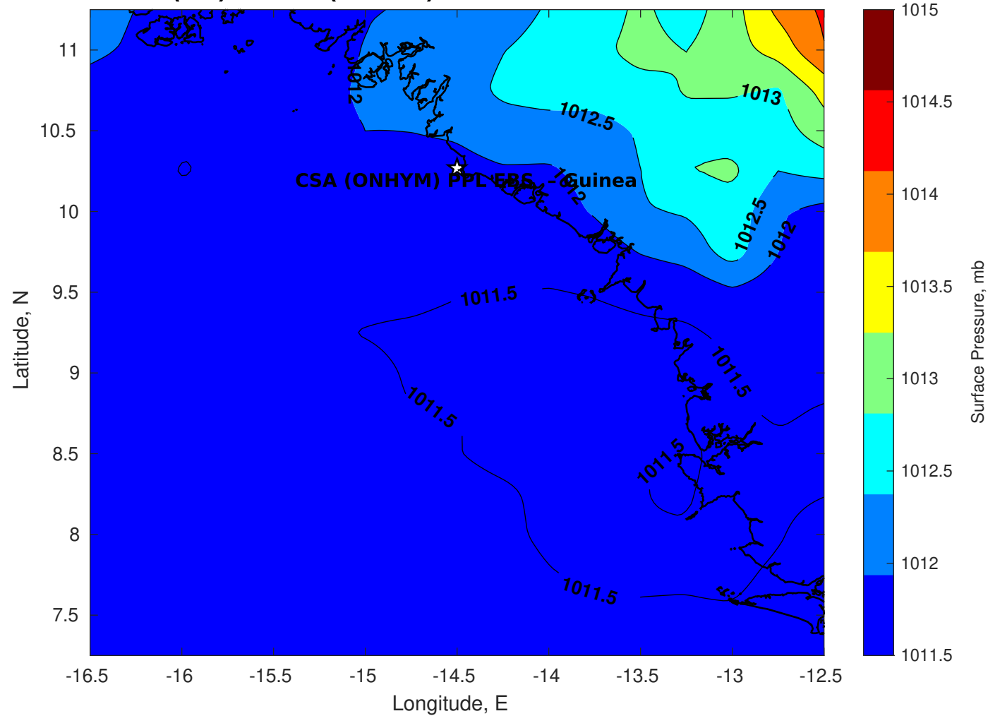
Surface Pressure (mb) for CSA (ONHYM) PPL EBS - Guinea at 26-Nov-2025 00:00:00
