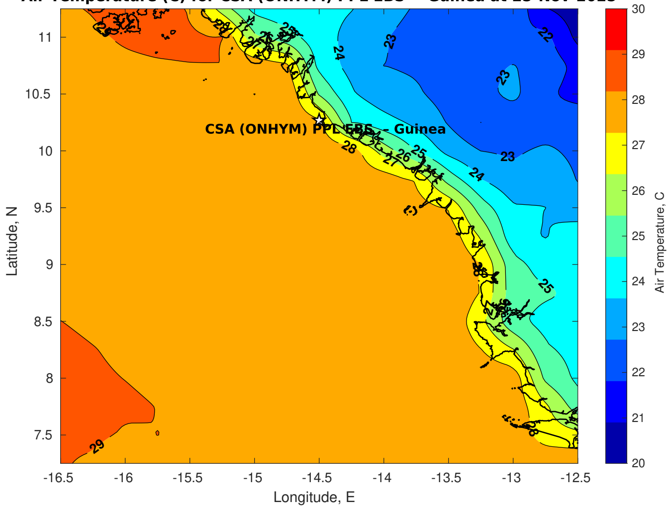
Air Temperature (C) for CSA (ONHYM) PPL EBS - Guinea at 25-Nov-2025
