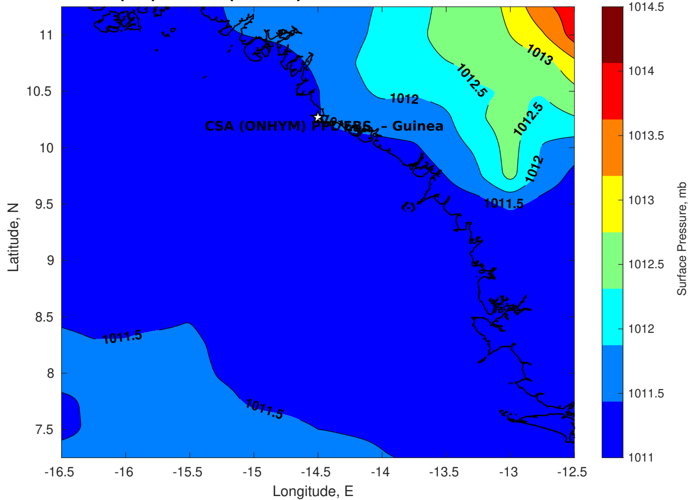
Surface Pressure (mb) for CSA (ONHYM) PPL EBS - Guinea at 27-Nov-2025 00:00:00
