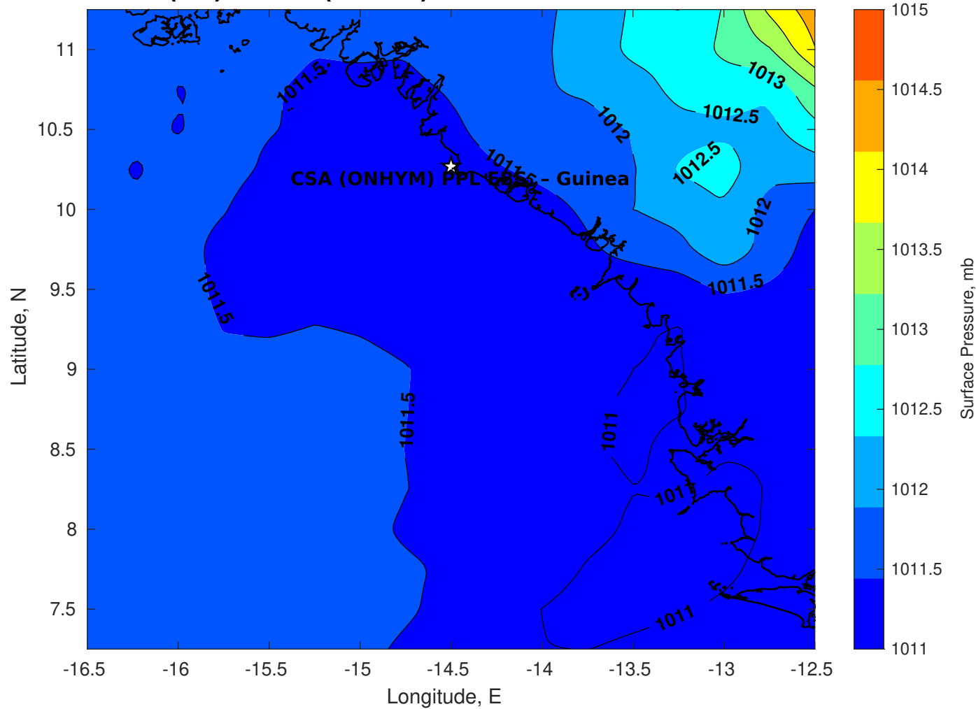
Surface Pressure (mb) for CSA (ONHYM) PPL EBS - Guinea at 25-Nov-2025 00:00:00
