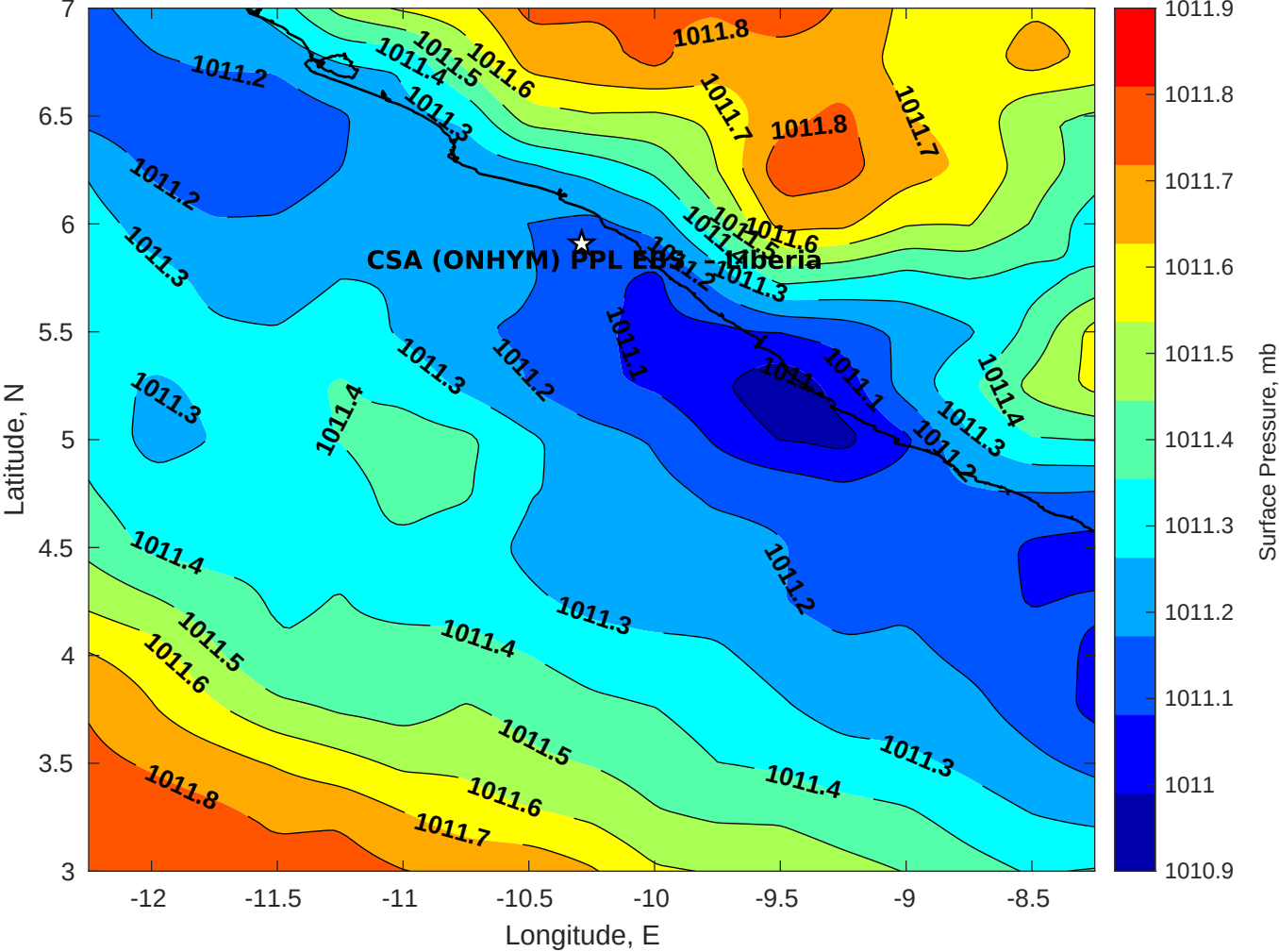
Surface Pressure (mb) for CSA (ONHYM) PPL EBS - Liberia at 27-Nov-2025 00:00:00
