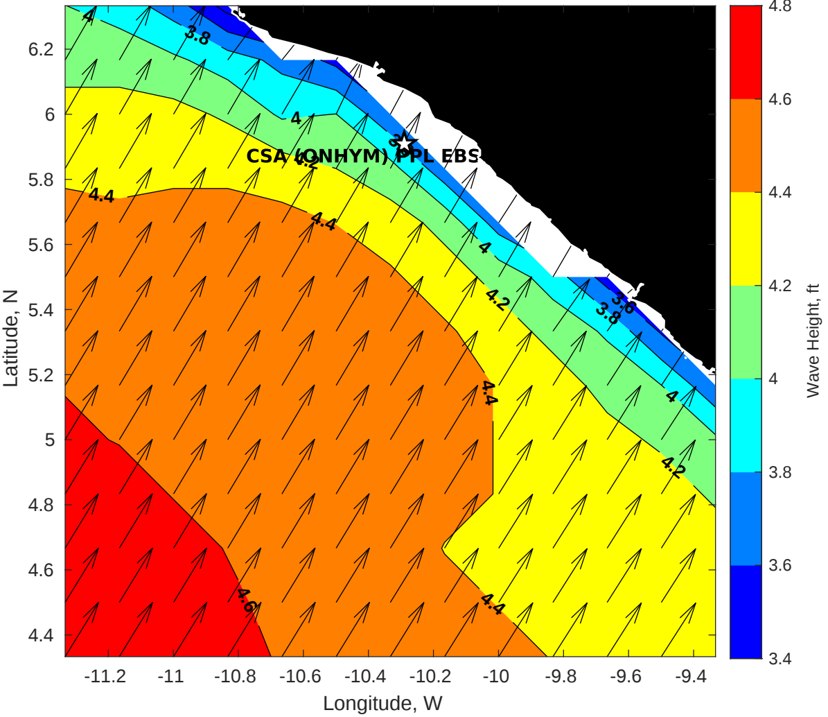
GFS Wave Height (ft) for CSA (ONHYM) PPL EBS - Liberia at 25-Nov-2025 09:00:00
