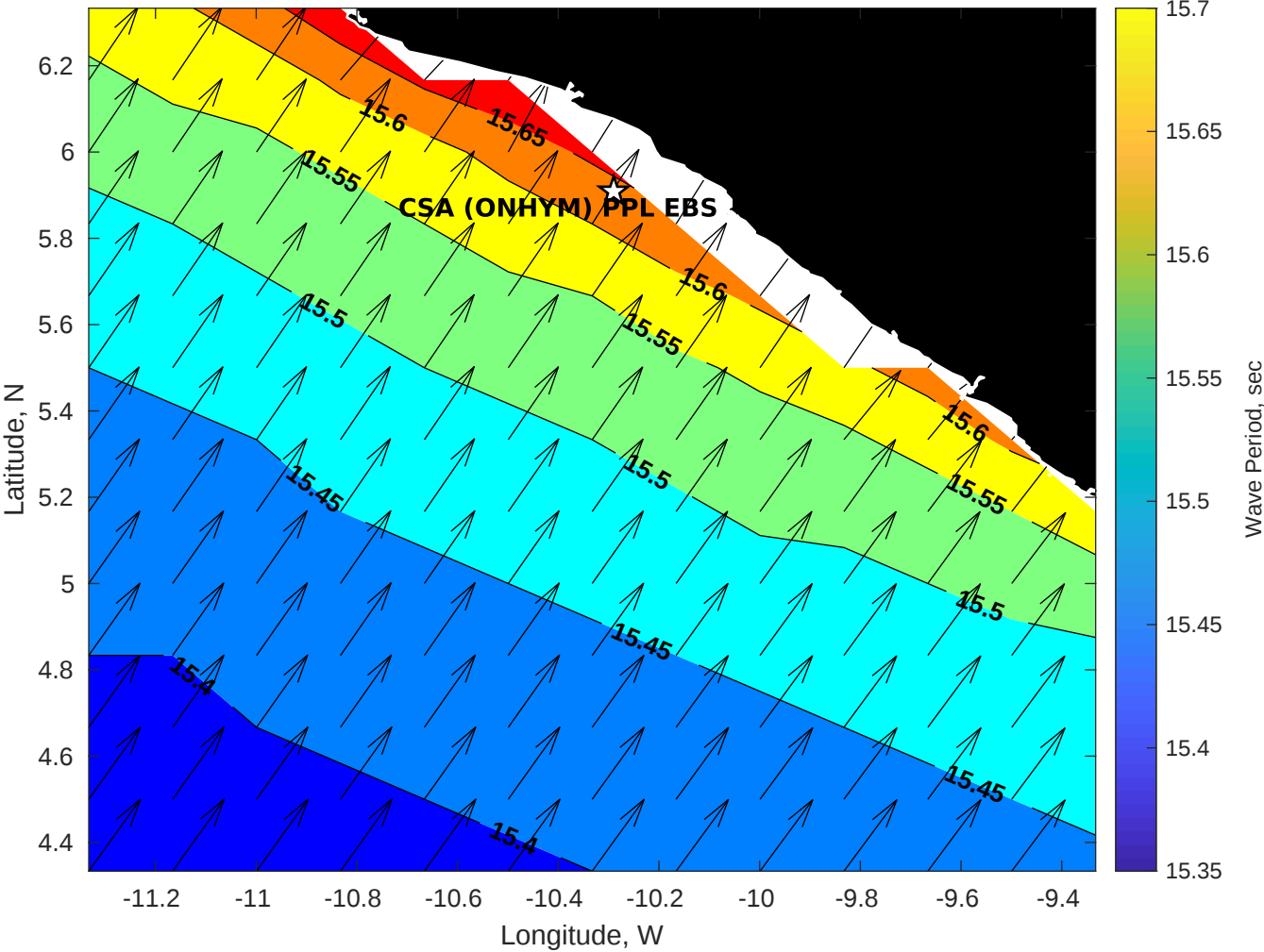
GFS Wave Period (sec) for CSA (ONHYM) PPL EBS - Liberia at 25-Nov-2025 09:00:00
