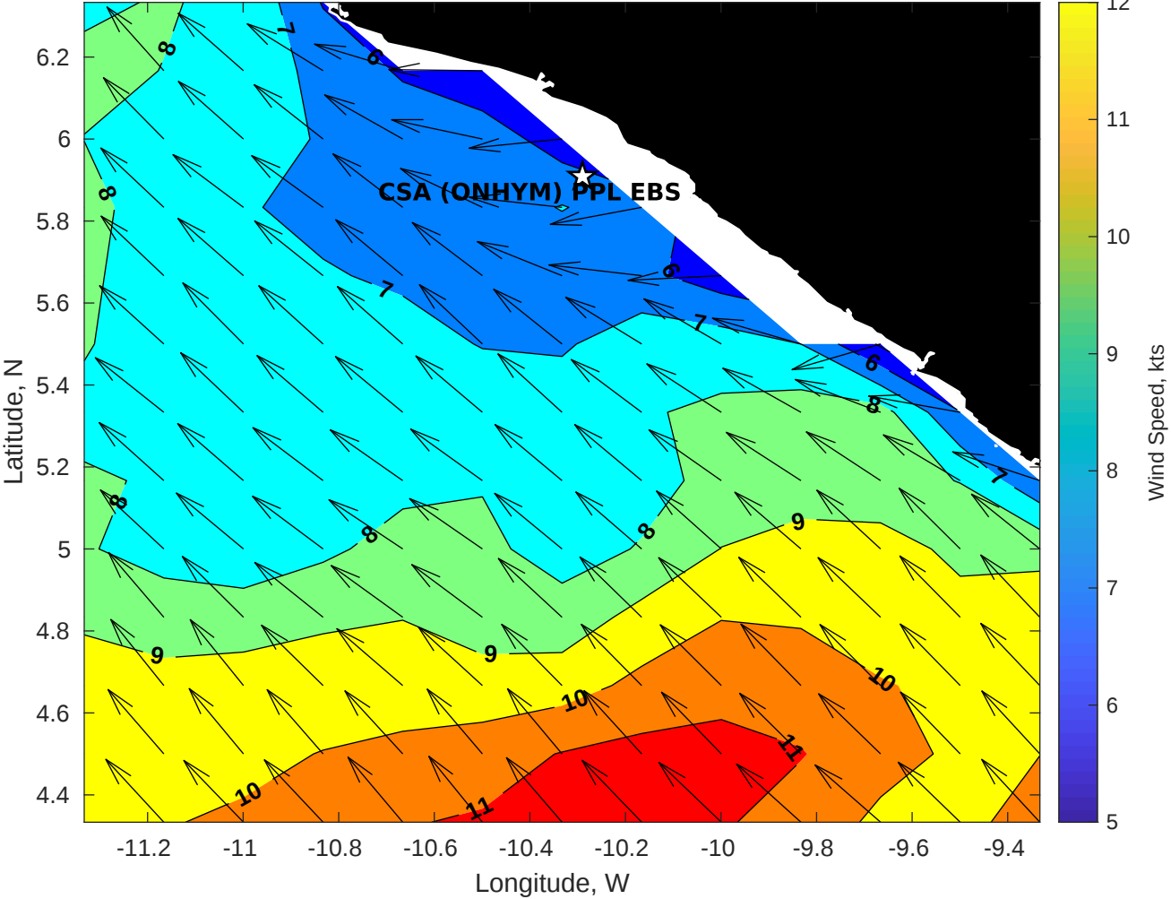
GFS Winds (kts) for CSA (ONHYM) PPL EBS - Liberia at 25-Nov-2025 09:00:00
