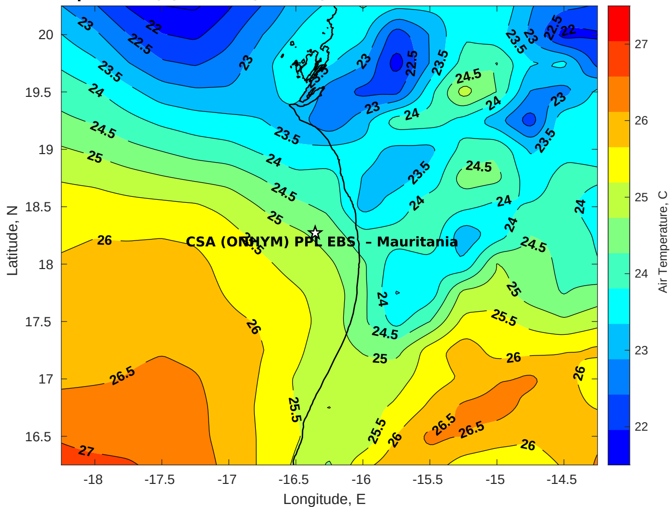
Air Temperature (C) for CSA (ONHYM) PPL EBS - Mauritania at 25-Nov-2025
