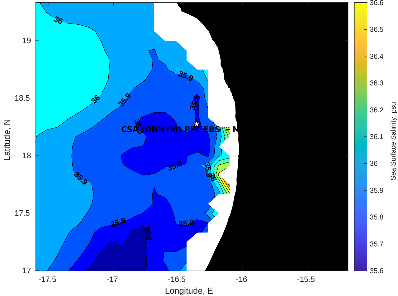
Surface Salinity for CSA (ONHYM) PPL EBS - Mauritania at 24-Nov-2025 00:00:00
