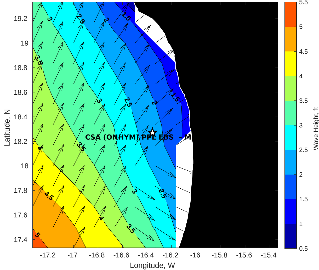
GFS Wave Height (ft) for CSA (ONHYM) PPL EBS - Mauritania at 25-Nov-2025 09:00:00
