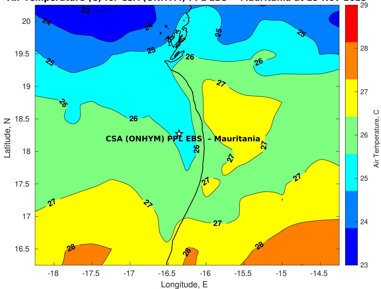
Air Temperature (C) for CSA (ONHYM) PPL EBS - Mauritania at 25-Nov-2025
