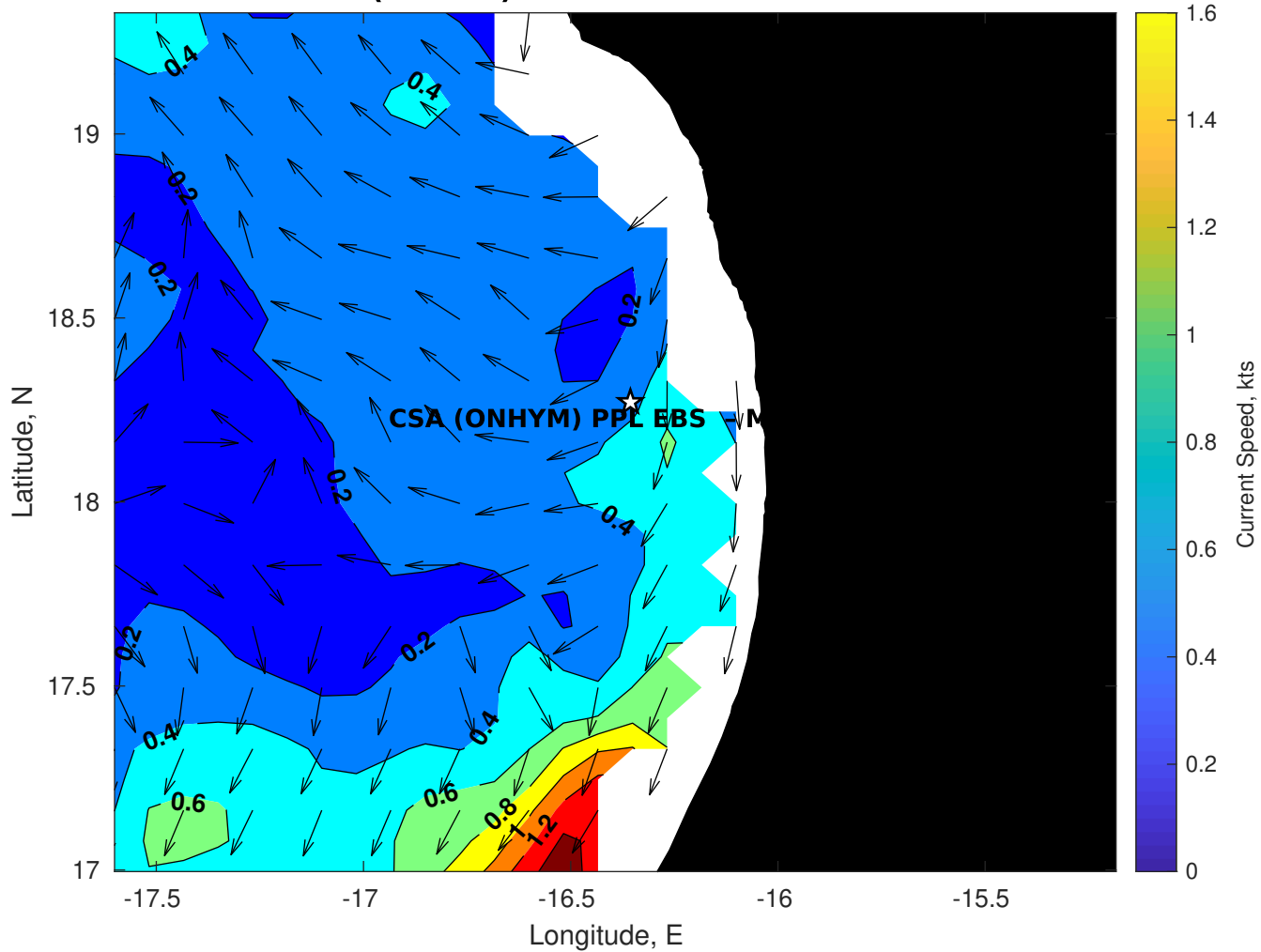
Surface Currents for CSA (ONHYM) PPL EBS - Mauritania at 24-Nov-2025 00:00:00
