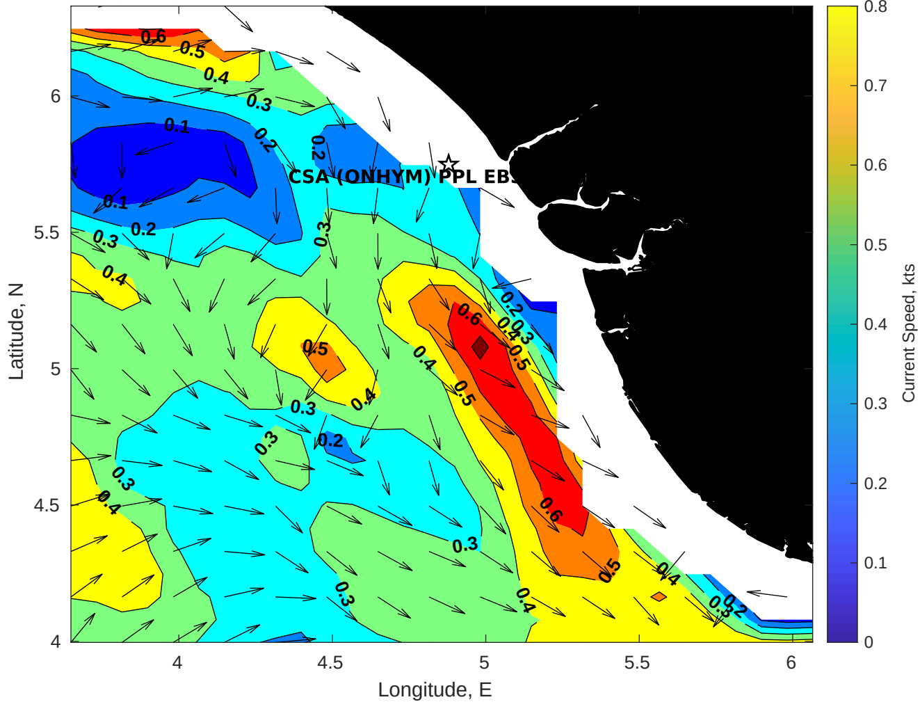
Surface Currents for CSA (ONHYM) PPL EBS - Nigeria at 24-Nov-2025 00:00:00
