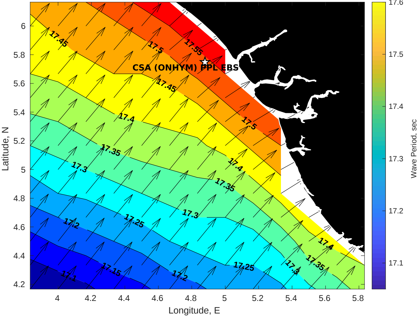
GFS Wave Period (sec) for CSA (ONHYM) PPL EBS - Nigeria at 25-Nov-2025 09:00:00
