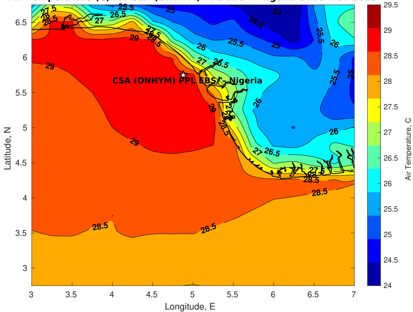
Air Temperature (C) for CSA (ONHYM) PPL EBS - Nigeria at 25-Nov-2025
