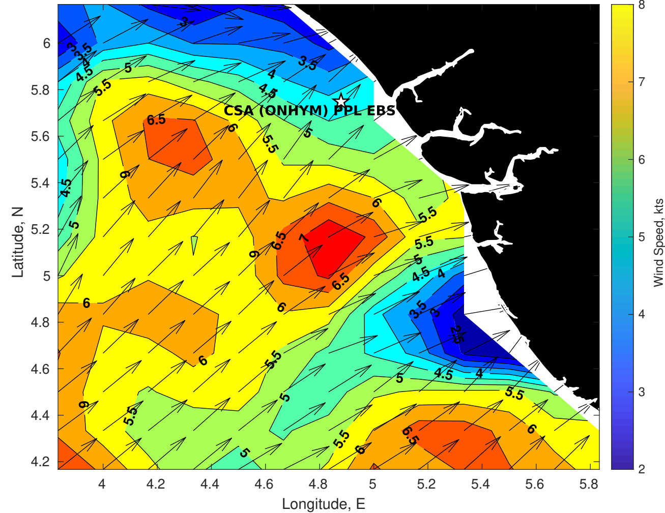
GFS Winds (kts) for CSA (ONHYM) PPL EBS - Nigeria at 25-Nov-2025 09:00:00
