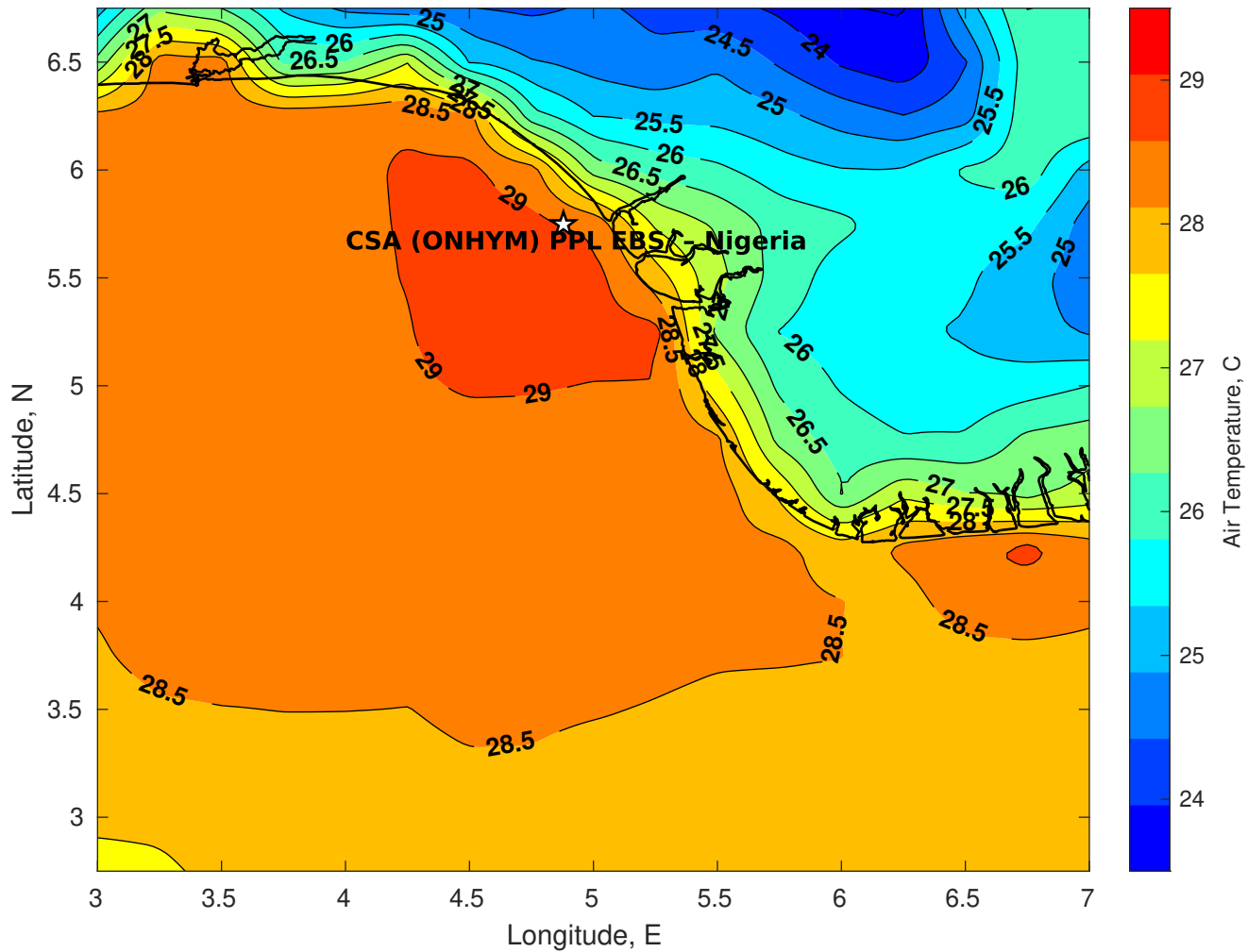
Air Temperature (C) for CSA (ONHYM) PPL EBS - Nigeria at 25-Nov-2025
