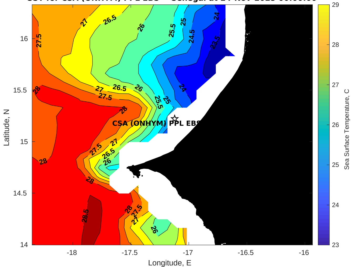
SST for CSA (ONHYM) PPL EBS - Senegal at 24-Nov-2025 00:00:00
