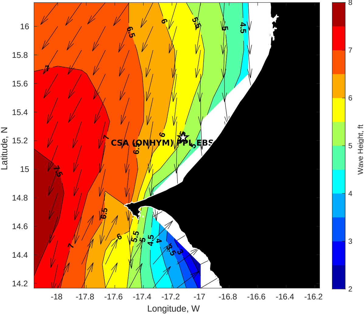
GFS Wave Height (ft) for CSA (ONHYM) PPL EBS - Senegal at 25-Nov-2025 09:00:00
