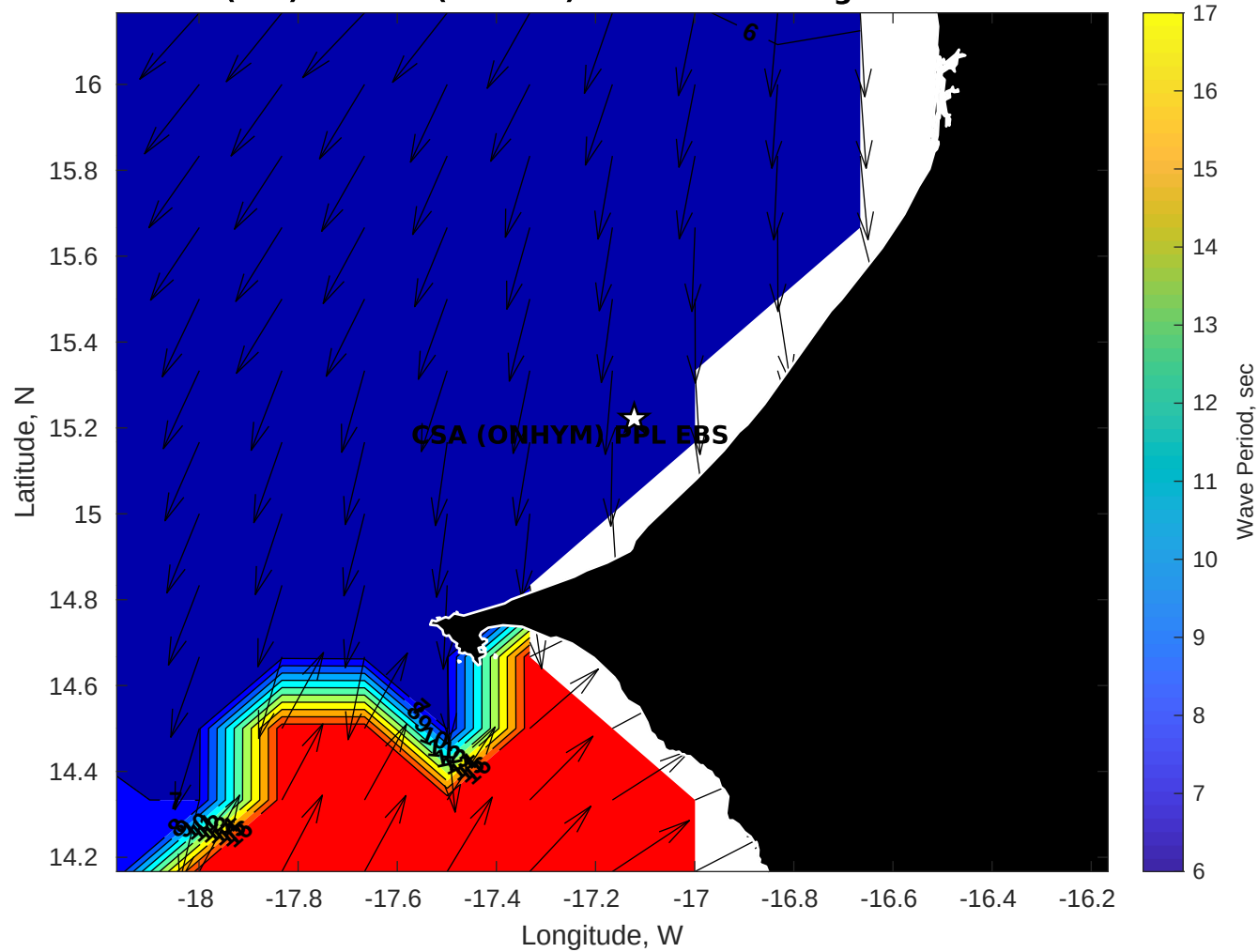
GFS Wave Period (sec) for CSA (ONHYM) PPL EBS - Senegal at 25-Nov-2025 09:00:00
