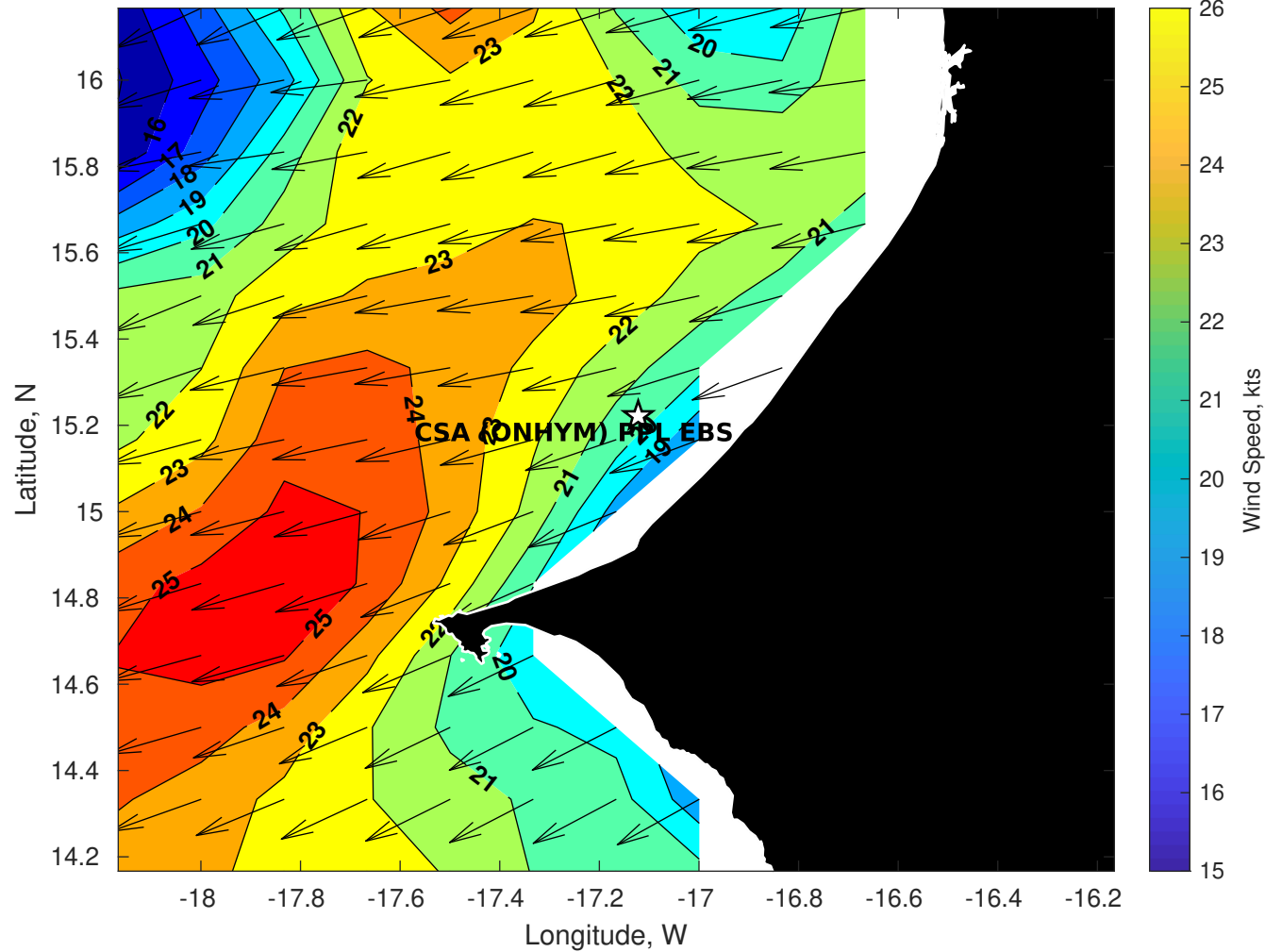
GFS Winds (kts) for CSA (ONHYM) PPL EBS - Senegal at 25-Nov-2025 09:00:00
