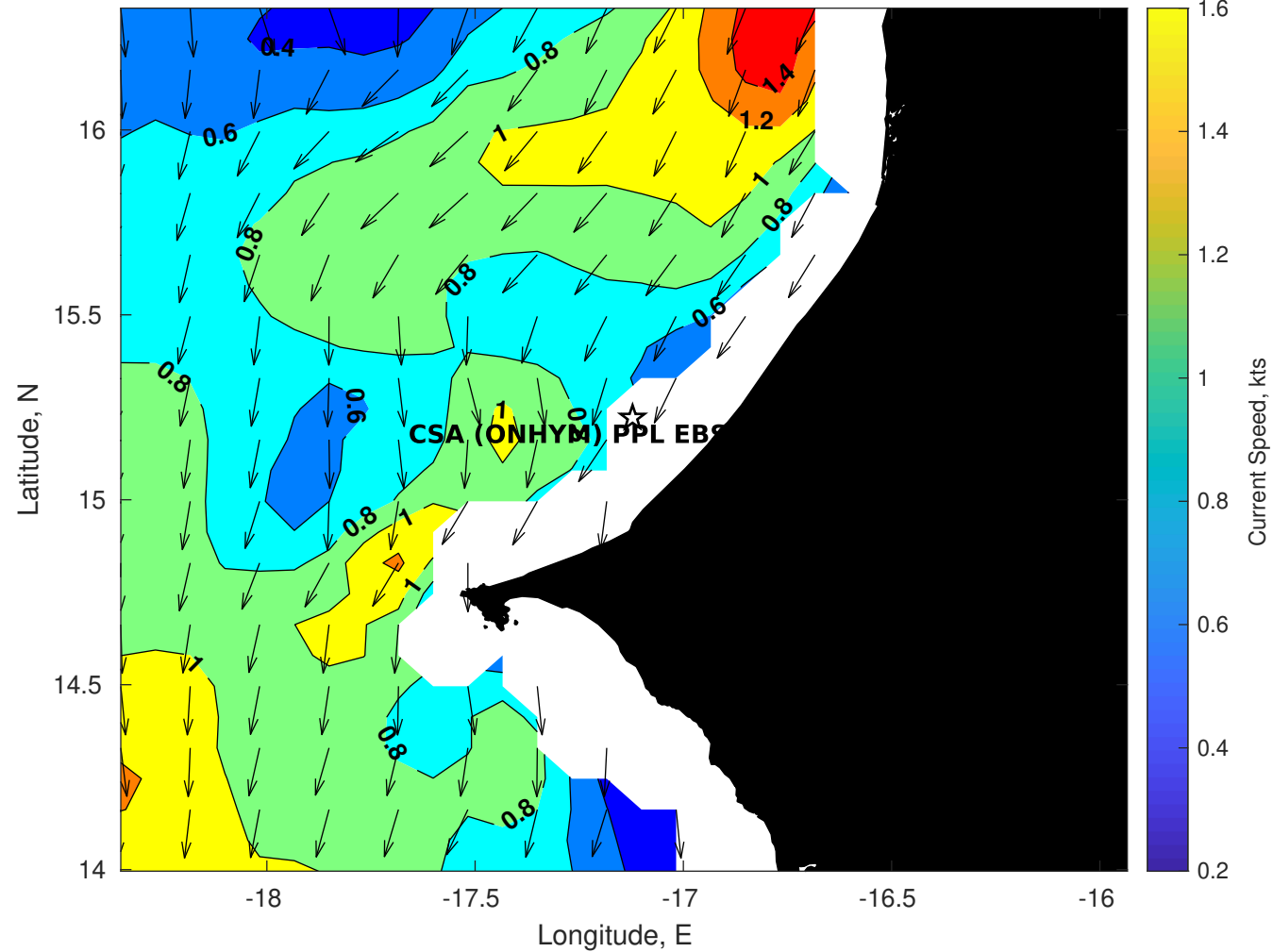
Surface Currents for CSA (ONHYM) PPL EBS - Senegal at 24-Nov-2025 00:00:00
