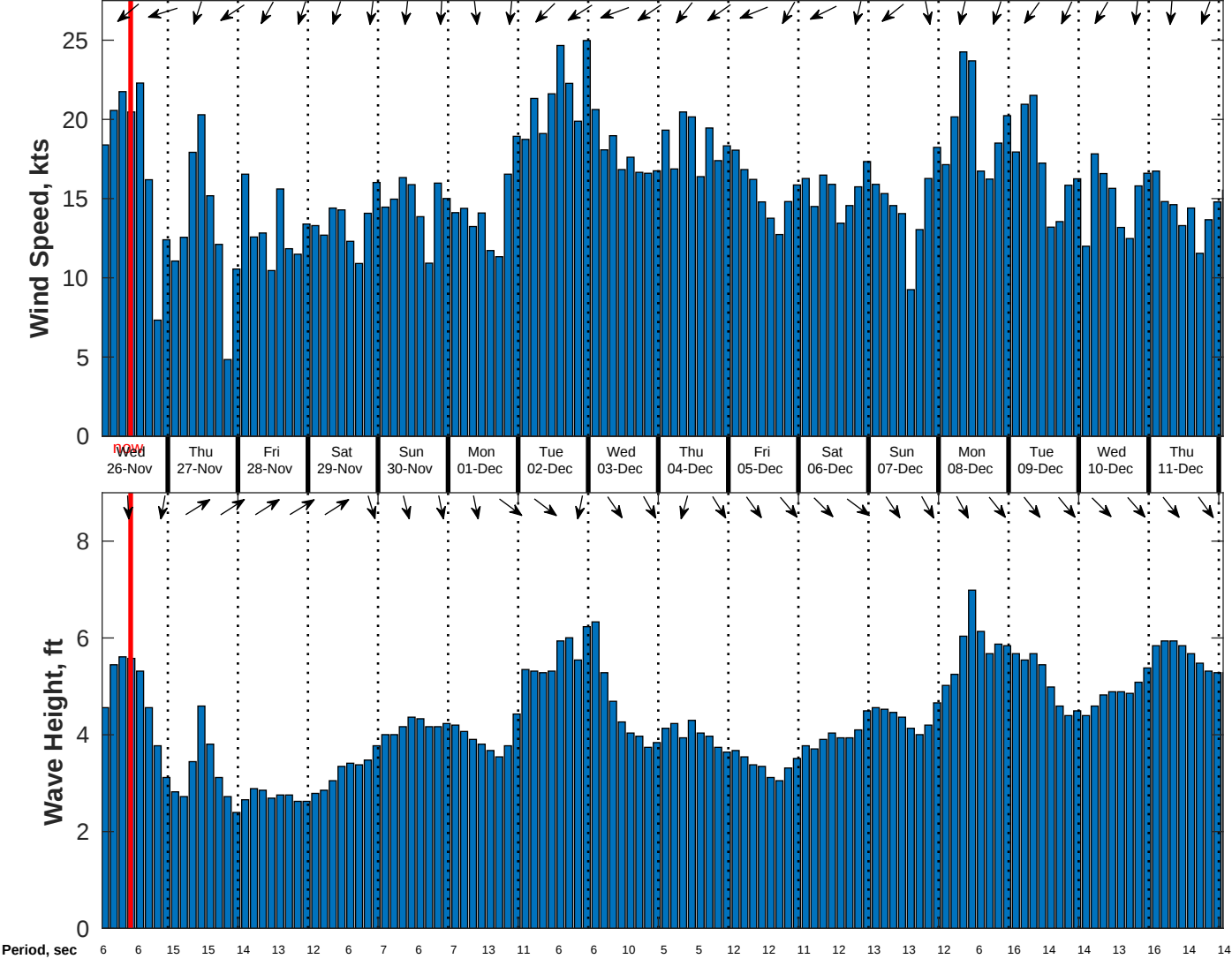
Wind & Wave Forecast for CSA (ONHYM) PPL EBS - Senegal from 25-Nov-2025 01:00:00 to 11-Dec-2025 01:00:00
