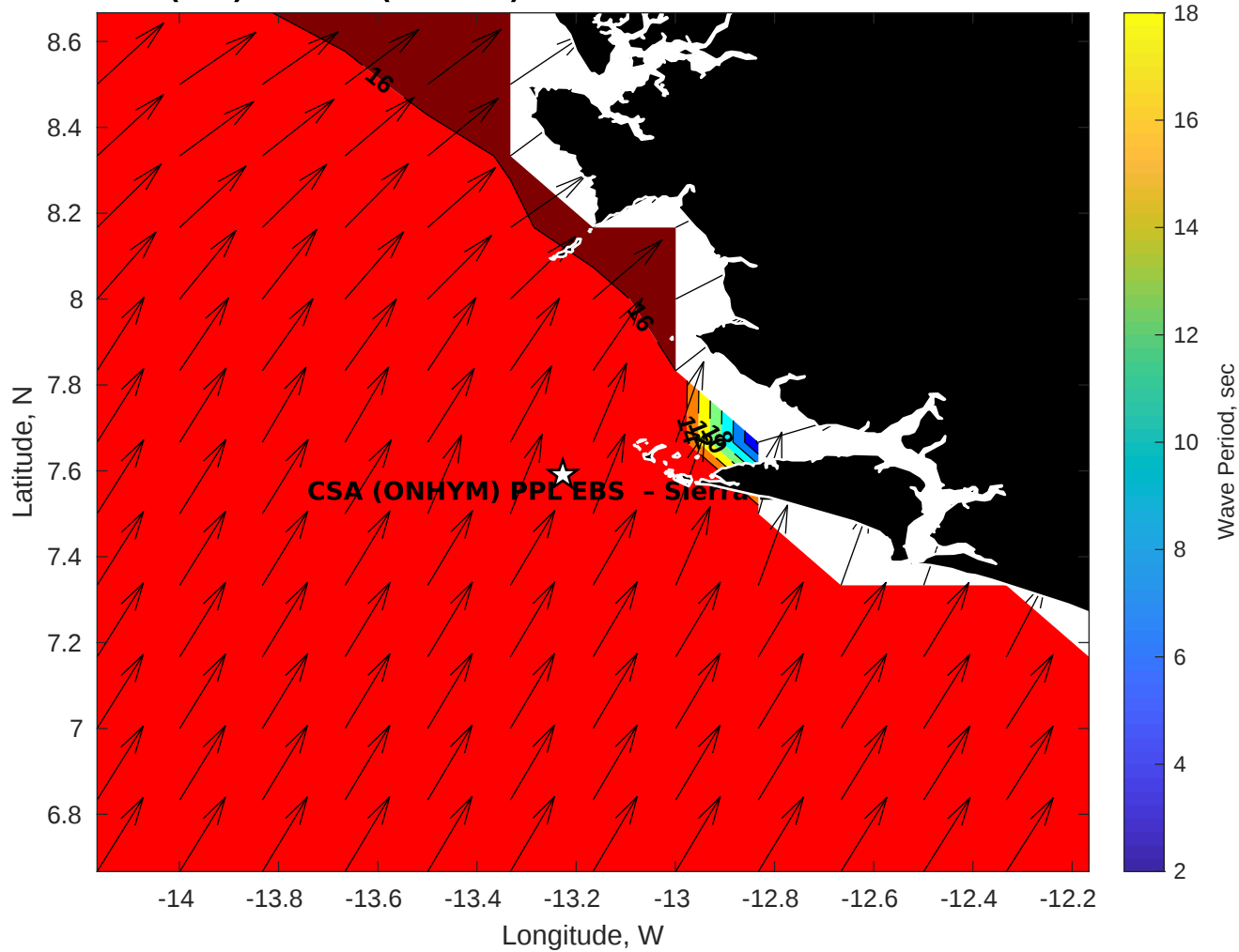
GFS Wave Period (sec) for CSA (ONHYM) PPL EBS - Sierra Leone at 25-Nov-2025 09:00:00
