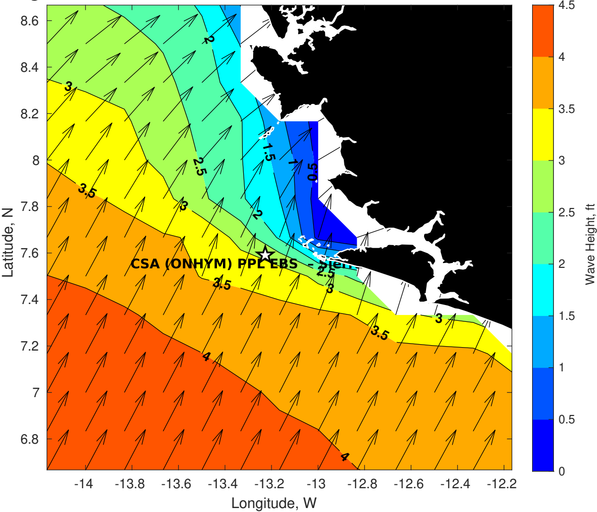
GFS Wave Height (ft) for CSA (ONHYM) PPL EBS - Sierra Leone at 25-Nov-2025 09:00:00
