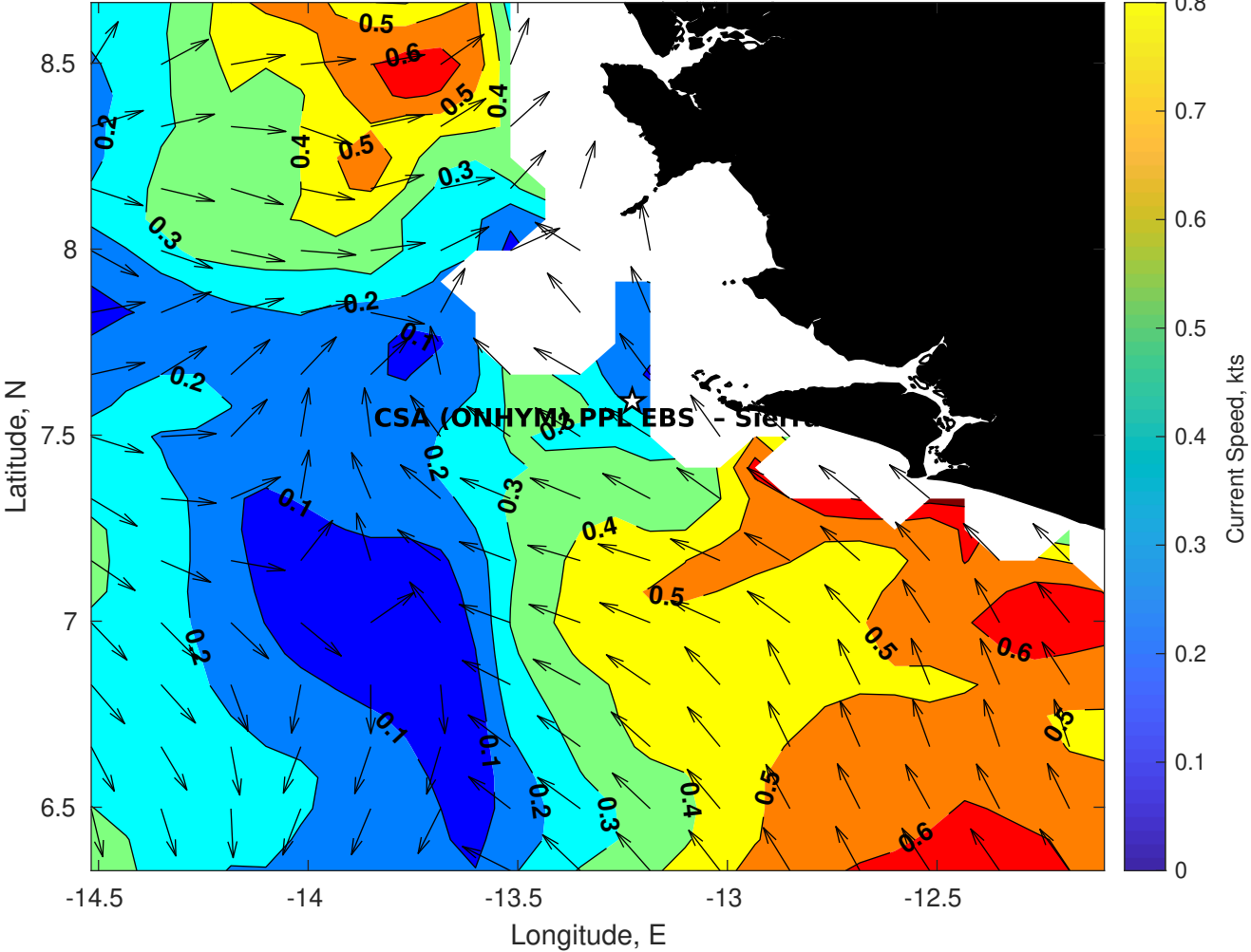
Surface Currents for CSA (ONHYM) PPL EBS - Sierra Leone at 24-Nov-2025 00:00:00
