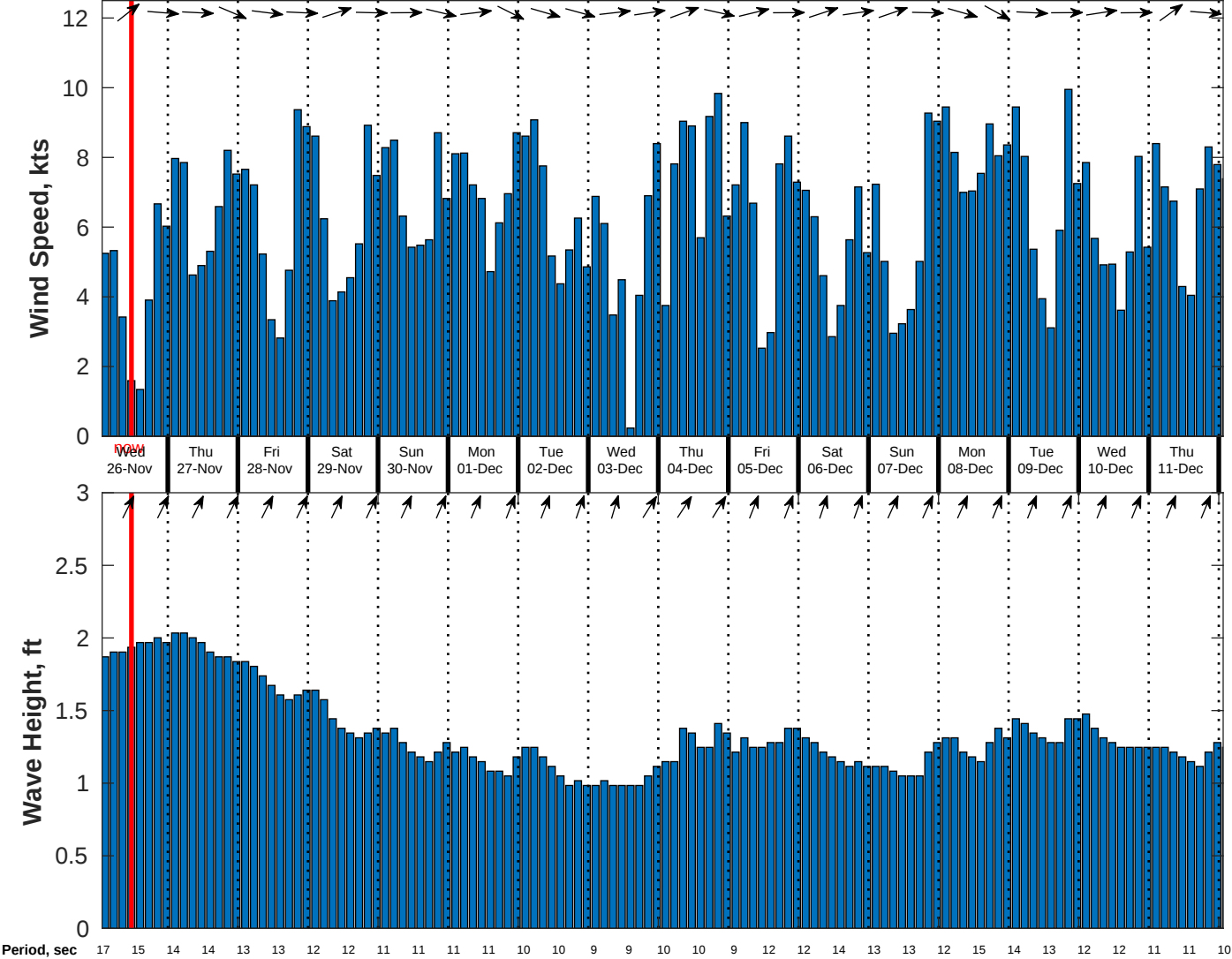
Wind & Wave Forecast for CSA (ONHYM) PPL EBS - Sierra Leone from 25-Nov-2025 01:00:00 to 11-Dec-2025 01:00:00
