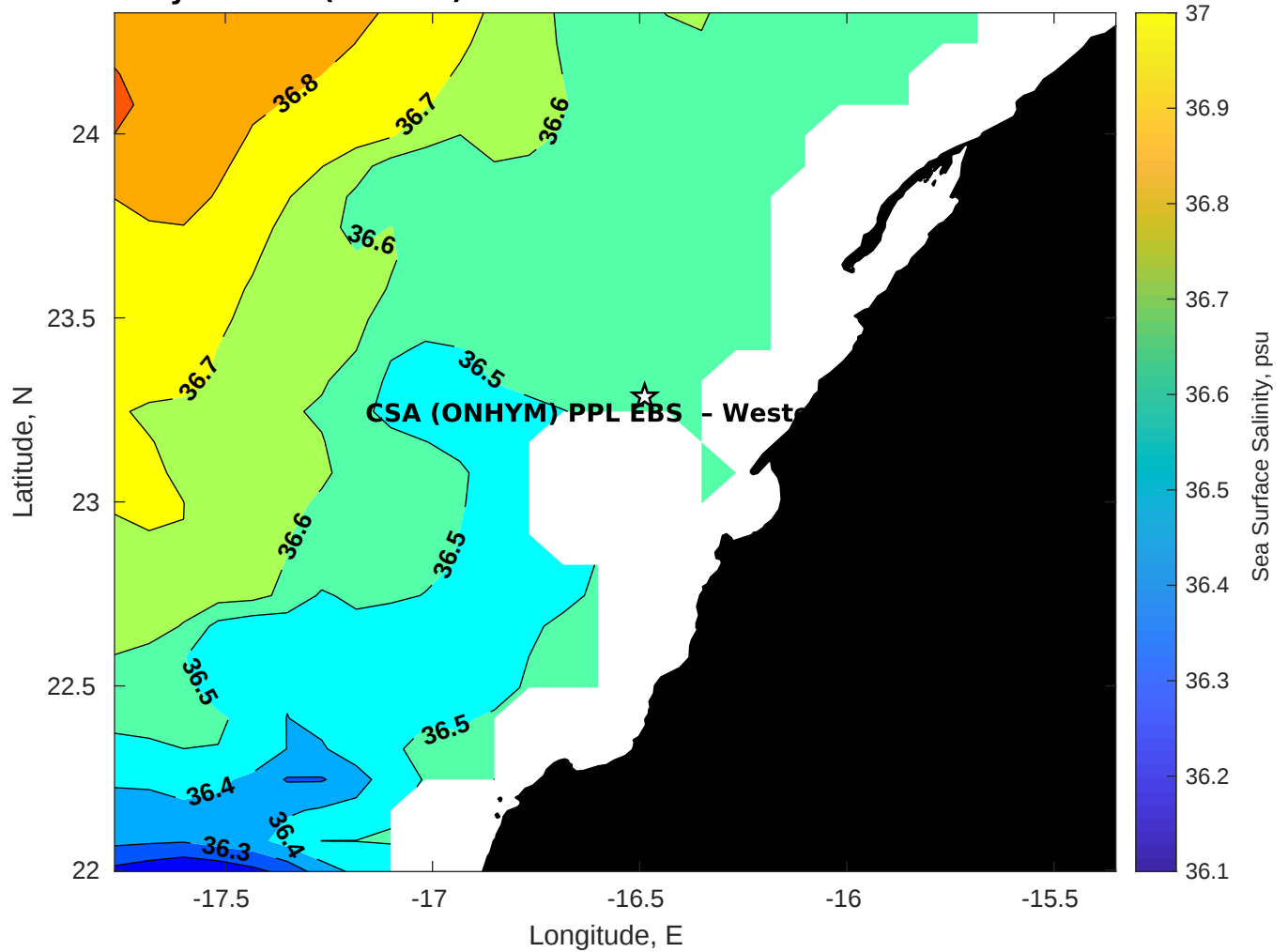
Surface Salinity for CSA (ONHYM) PPL EBS - Western Sahara at 24-Nov-2025 00:00:00
