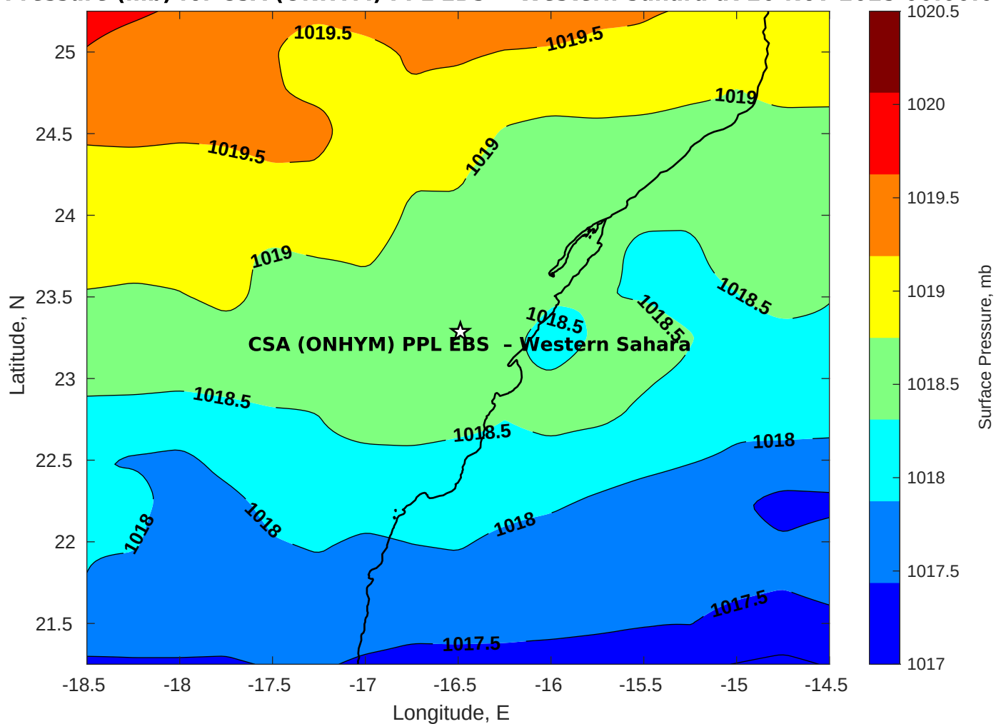
Surface Pressure (mb) for CSA (ONHYM) PPL EBS - Western Sahara at 26-Nov-2025 00:00:00
