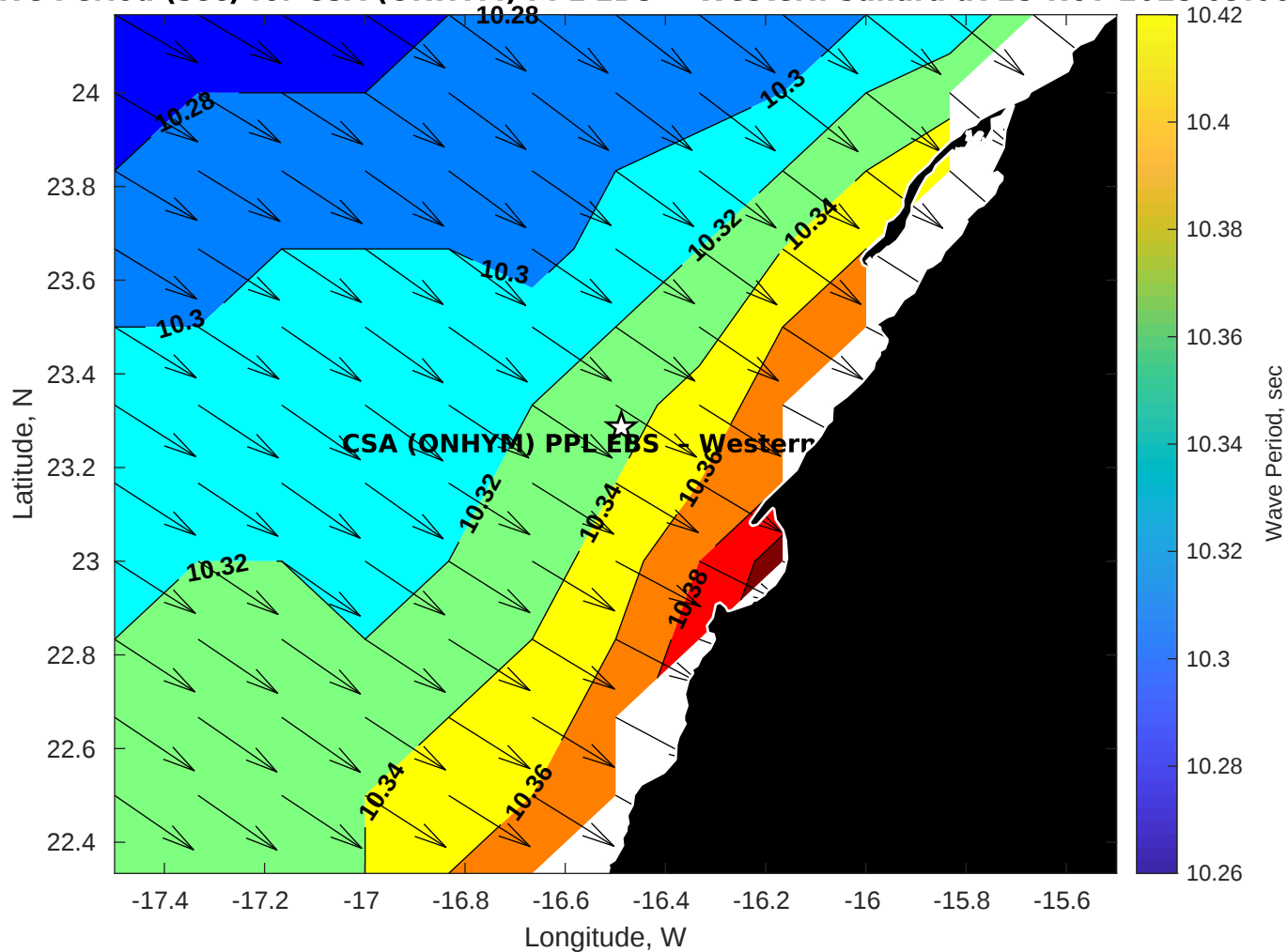
GFS Wave Period (sec) for CSA (ONHYM) PPL EBS - Western Sahara at 25-Nov-2025 09:00:00
