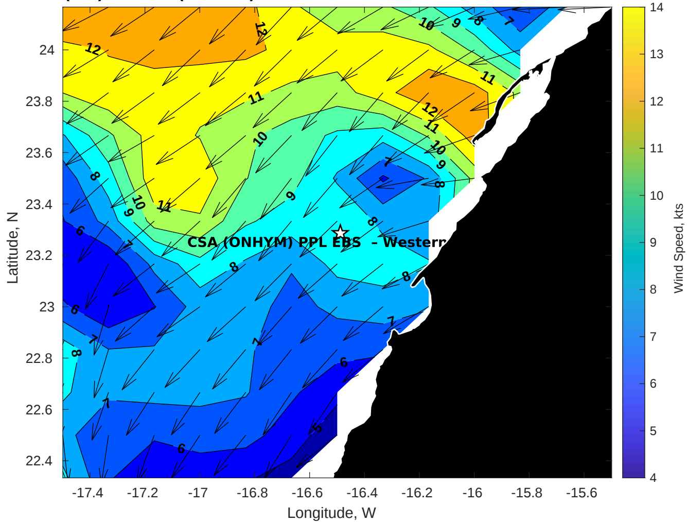
GFS Winds (kts) for CSA (ONHYM) PPL EBS - Western Sahara at 25-Nov-2025 09:00:00
