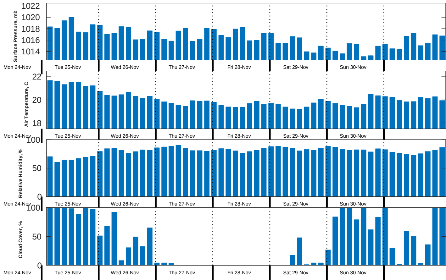
Met Forecast for CSA (ONHYM) PPL EBS - Western Sahara from 25-Nov-2025 00:00:00 to 02-Dec-2025 00:00:00
