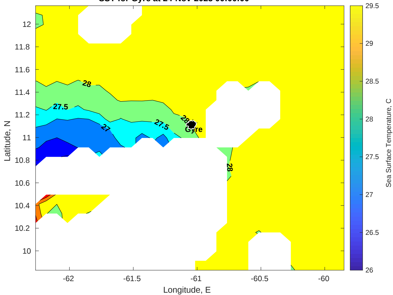
SST for Gyre at 24-Nov-2025 00:00:00
