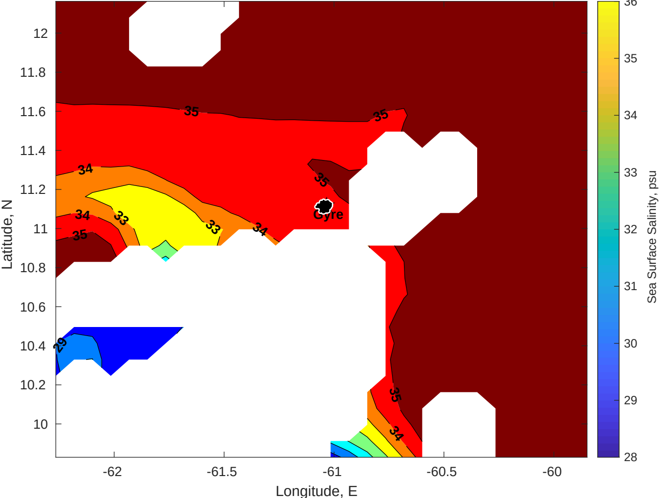
Surface Salinity for Gyre at 24-Nov-2025 00:00:00
