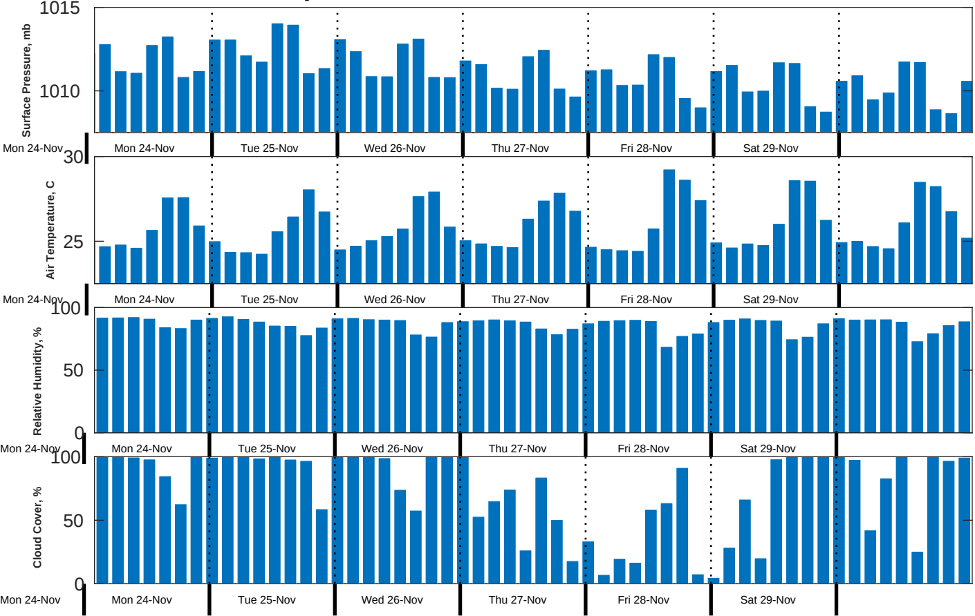
Met Forecast for Gyre from 24-Nov-2025 20:00:00 to 01-Dec-2025 20:00:00
