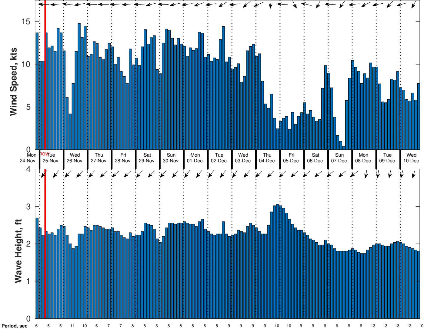
Wind & Wave Forecast for Gyre from 24-Nov-2025 20:00:00 to 10-Dec-2025 20:00:00
