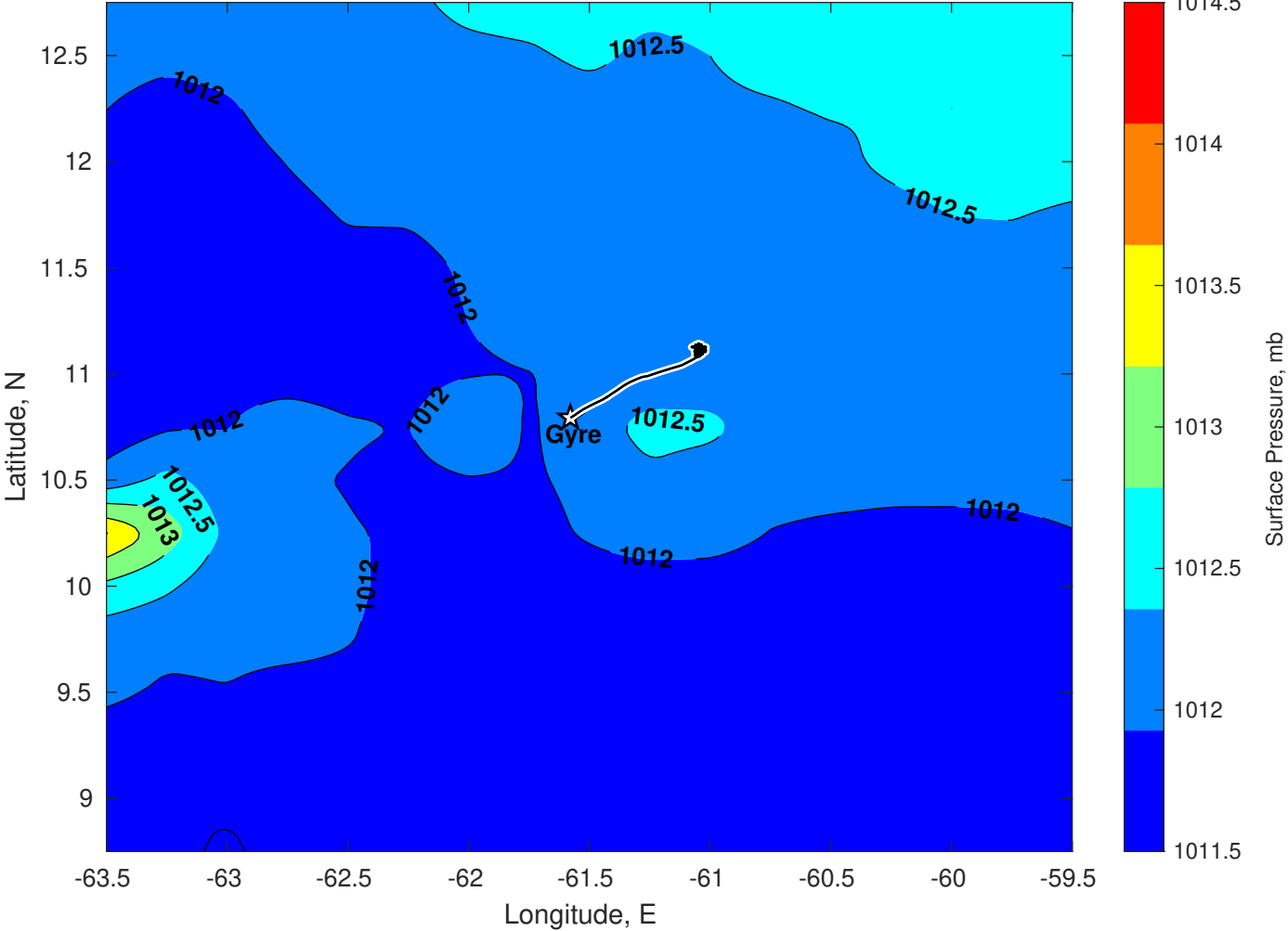
Surface Pressure (mb) for Gyre at 25-Nov-2025 00:00:00
