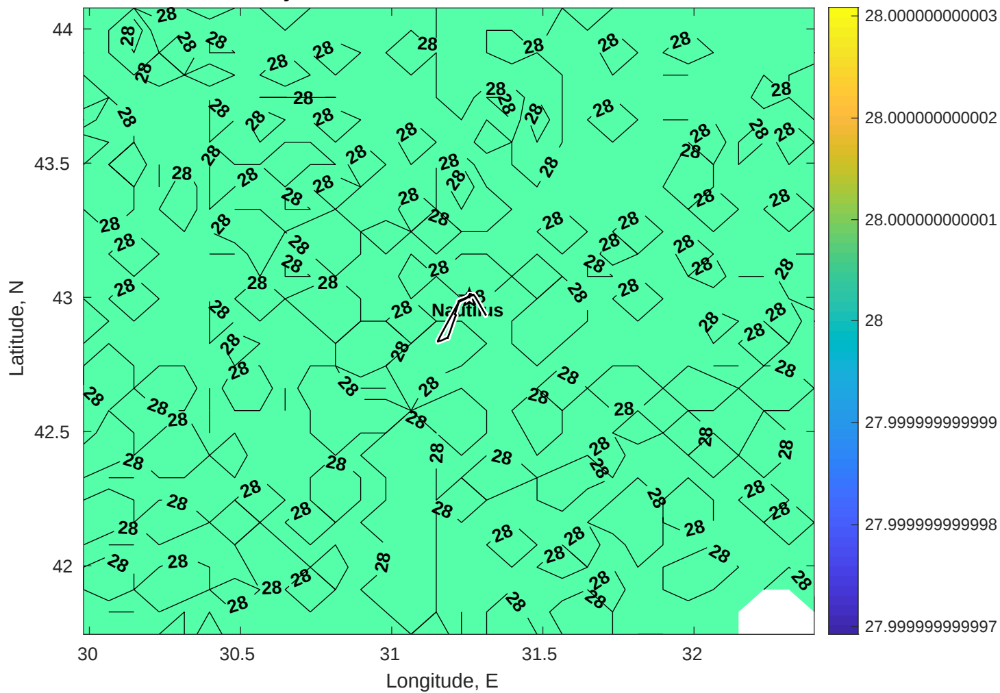
Surface Salinity for Nautilus at 24-Nov-2025 00:00:00
