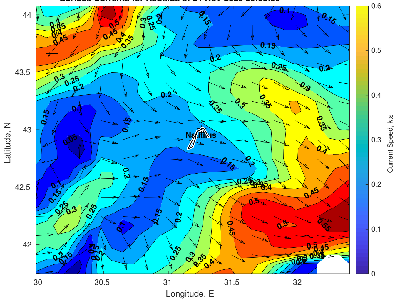
Surface Currents for Nautilus at 24-Nov-2025 00:00:00
