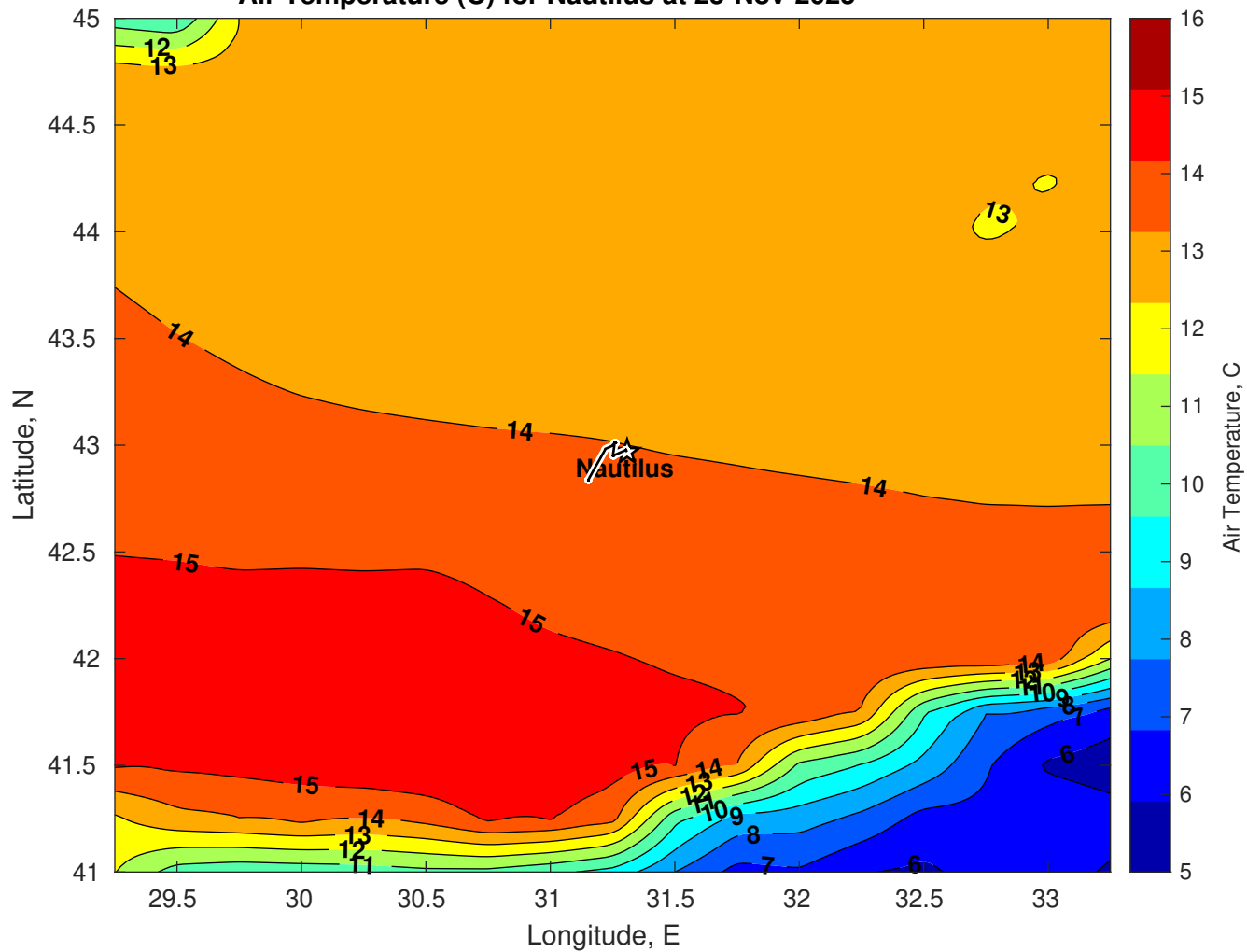
Air Temperature (C) for Nautilus at 25-Nov-2025
