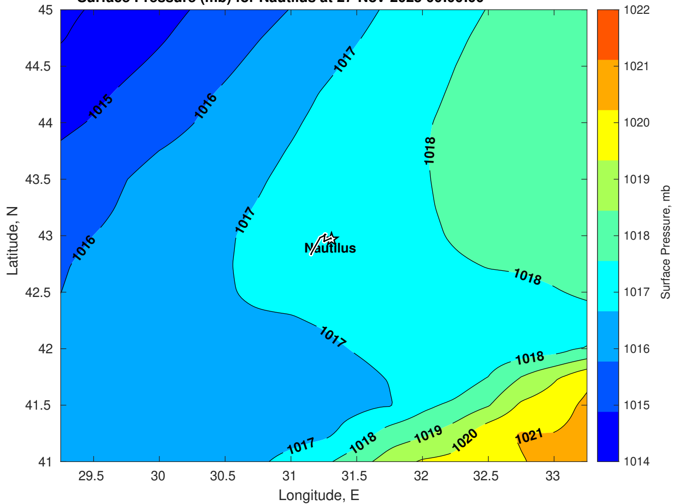
Surface Pressure (mb) for Nautilus at 27-Nov-2025 00:00:00
