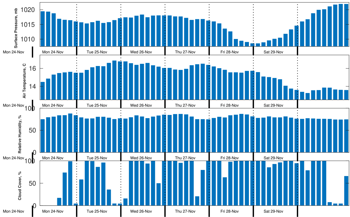
Met Forecast for Nautilus from 25-Nov-2025 00:00:00 to 02-Dec-2025 00:00:00
