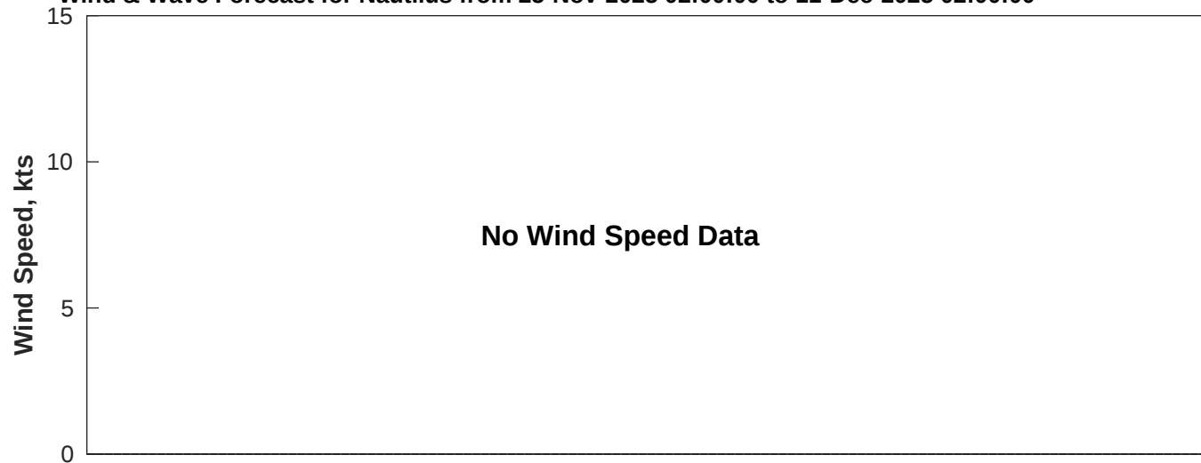
Wind & Wave Forecast for Nautilus from 25-Nov-2025 02:00:00 to 11-Dec-2025 02:00:00
