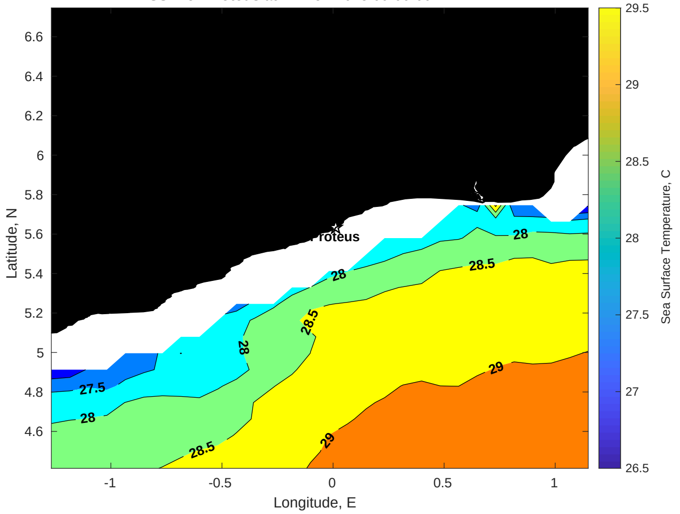
SST for Proteus at 24-Nov-2025 00:00:00
