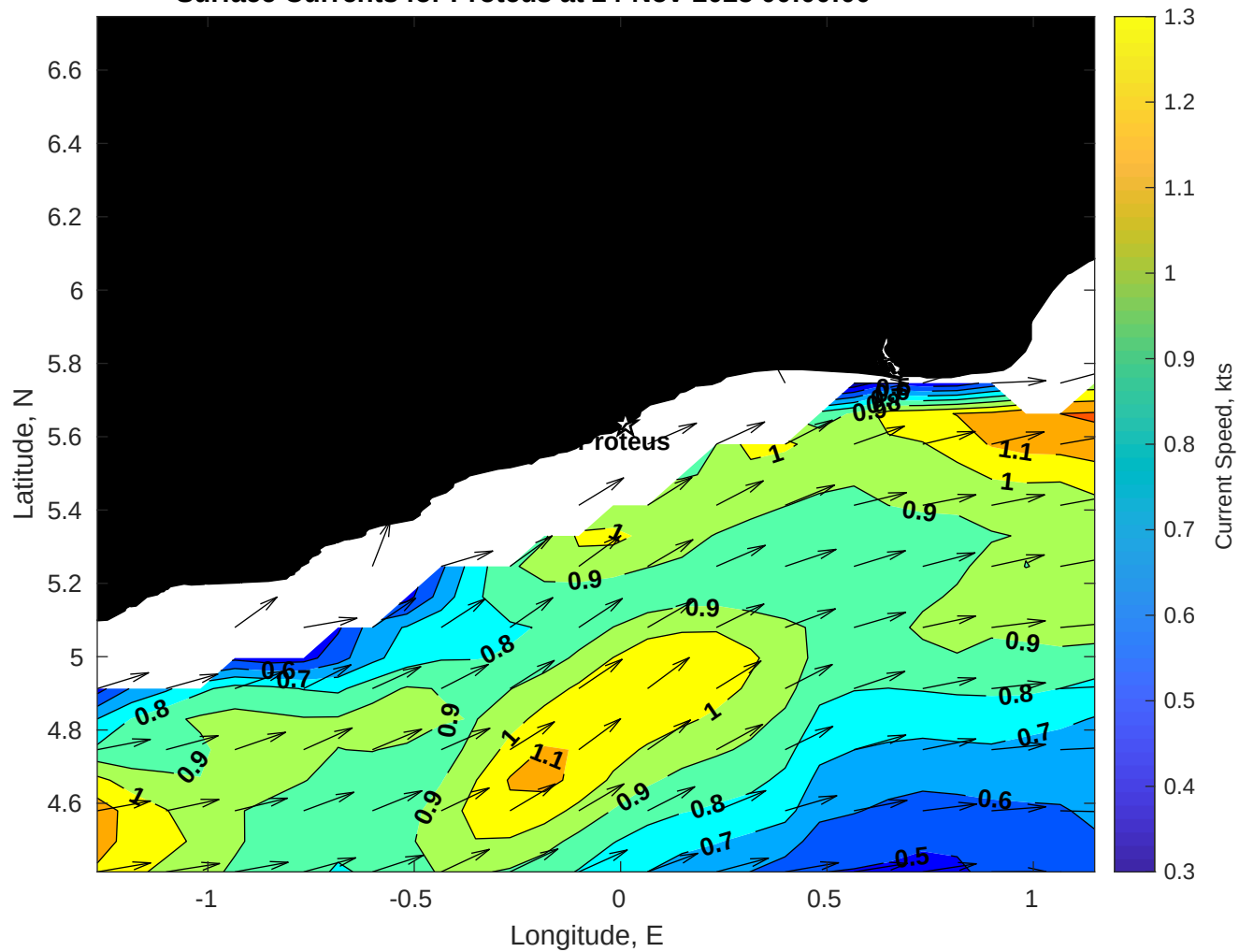
Surface Currents for Proteus at 24-Nov-2025 00:00:00
