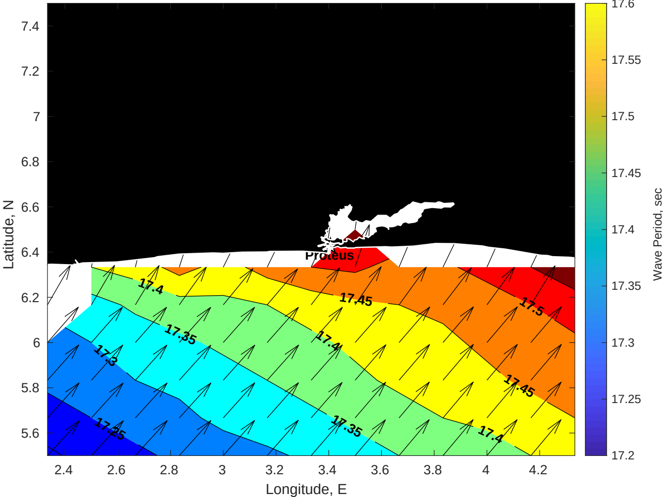
GFS Wave Period (sec) for Proteus at 25-Nov-2025 09:00:00
