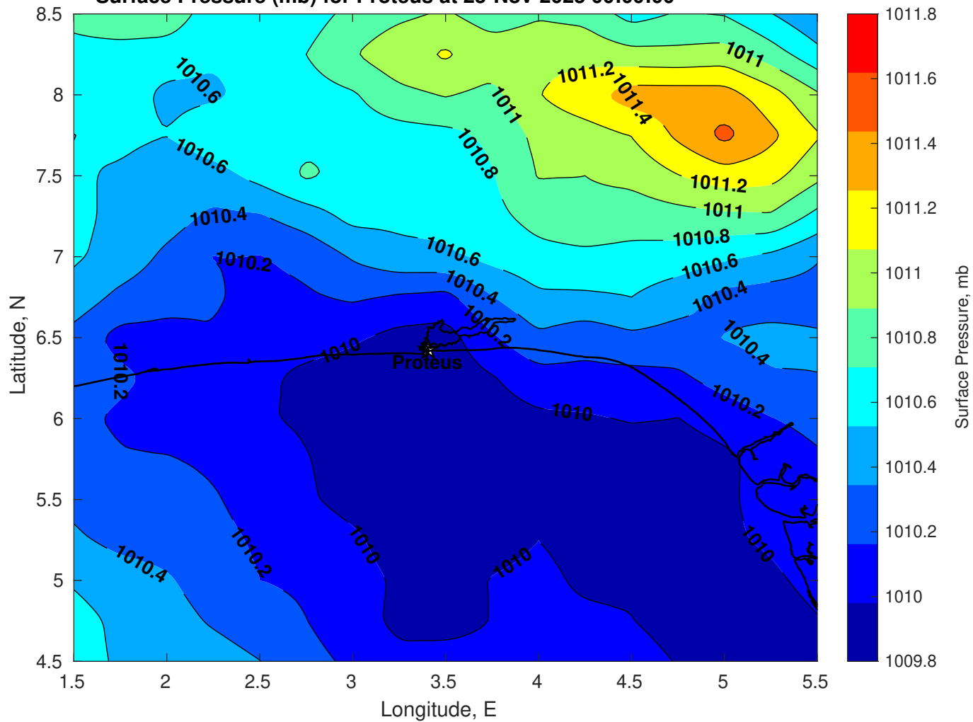
Surface Pressure (mb) for Proteus at 25-Nov-2025 00:00:00
