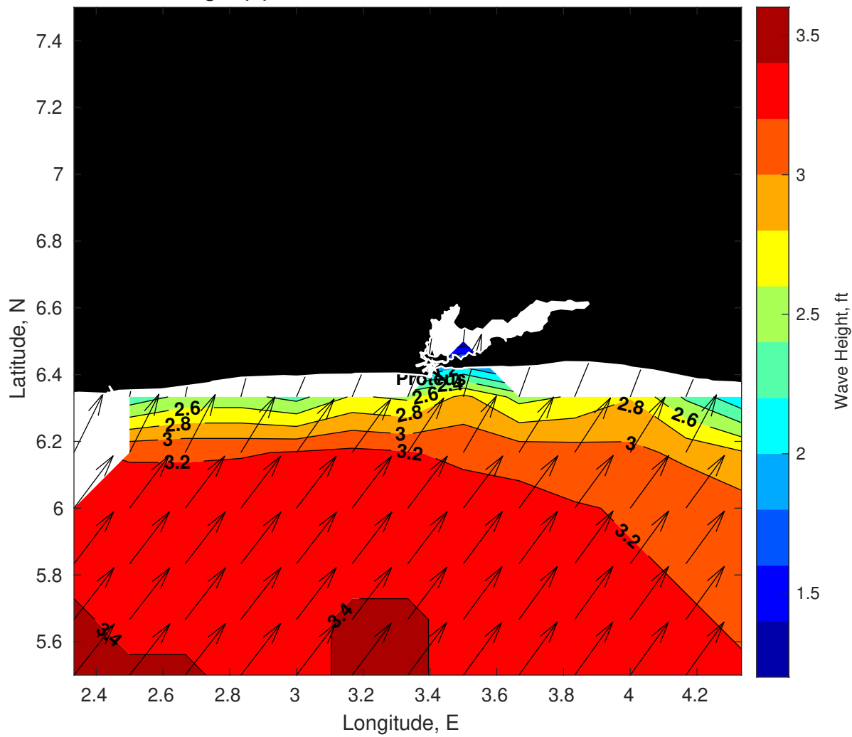
GFS Wave Height (ft) for Proteus at 25-Nov-2025 09:00:00
