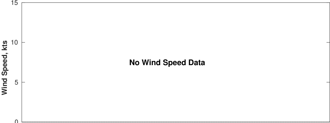
Wind & Wave Forecast for Proteus from 25-Nov-2025 01:00:00 to 11-Dec-2025 01:00:00
