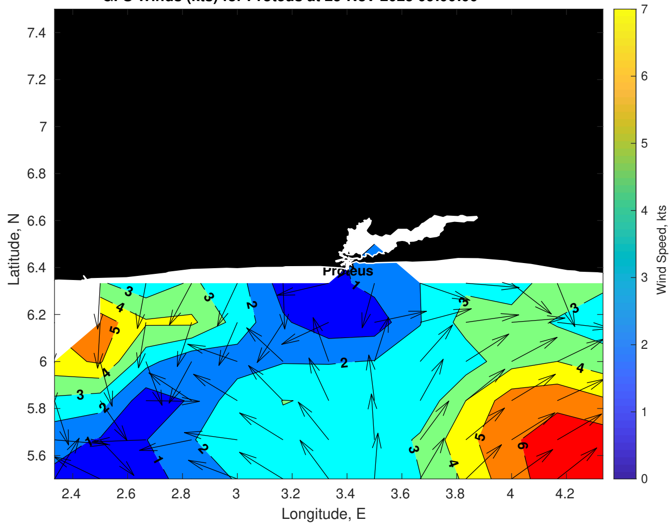
GFS Winds (kts) for Proteus at 25-Nov-2025 09:00:00
