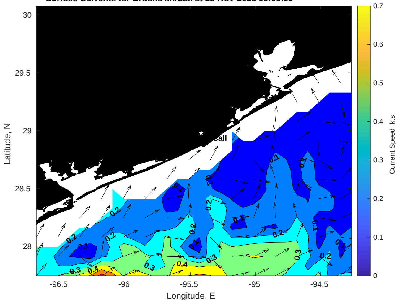
Surface Currents for Brooks McCall at 25-Nov-2025 00:00:00
