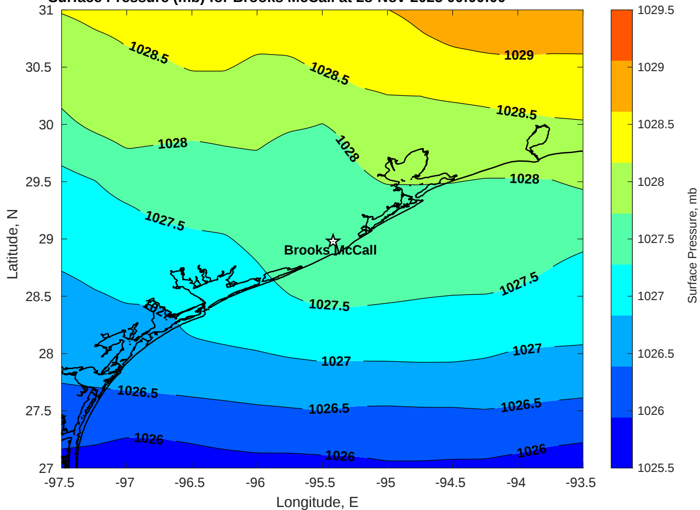
Surface Pressure (mb) for Brooks McCall at 28-Nov-2025 00:00:00
