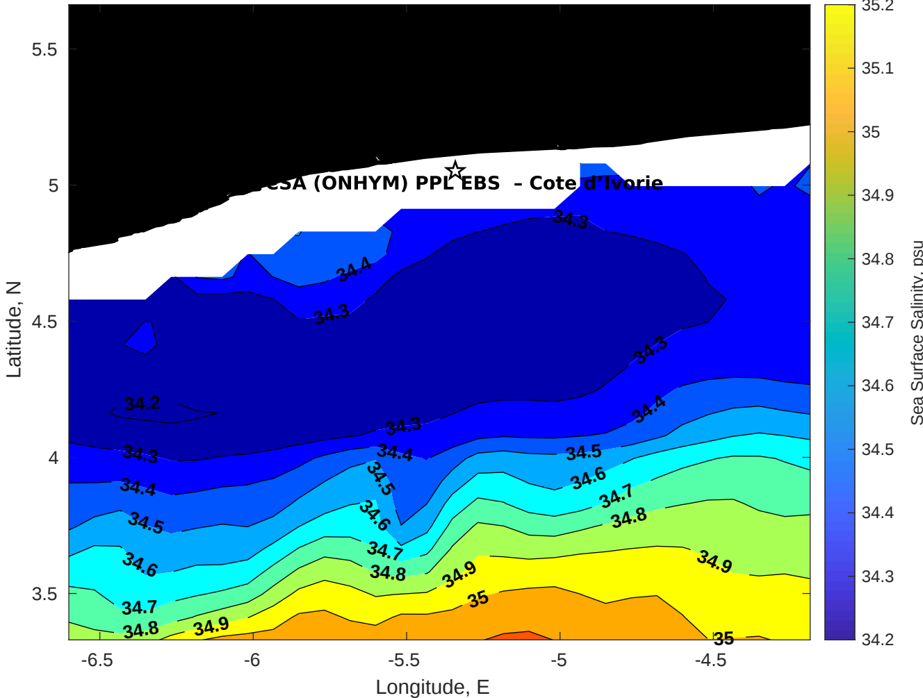
Surface Salinity for CSA (ONHYM) PPL EBS - Cote d'Ivoire at 25-Nov-2025 00:00:00
