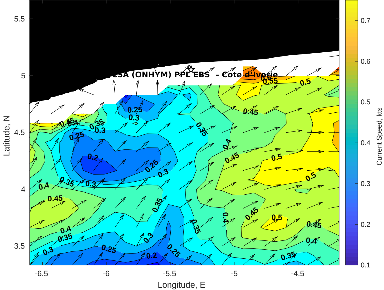
Surface Currents for CSA (ONHYM) PPL EBS - Cote d'Ivoire at 25-Nov-2025 00:00:00
