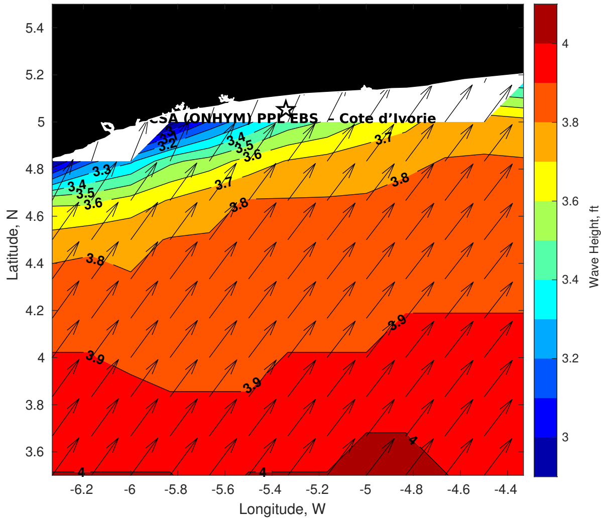
GFS Wave Height (ft) for CSA (ONHYM) PPL EBS - Cote d'Ivoire at 26-Nov-2025 09:00:00
