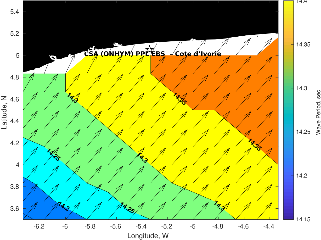
GFS Wave Period (sec) for CSA (ONHYM) PPL EBS - Cote d'Ivoire at 26-Nov-2025 09:00:00
