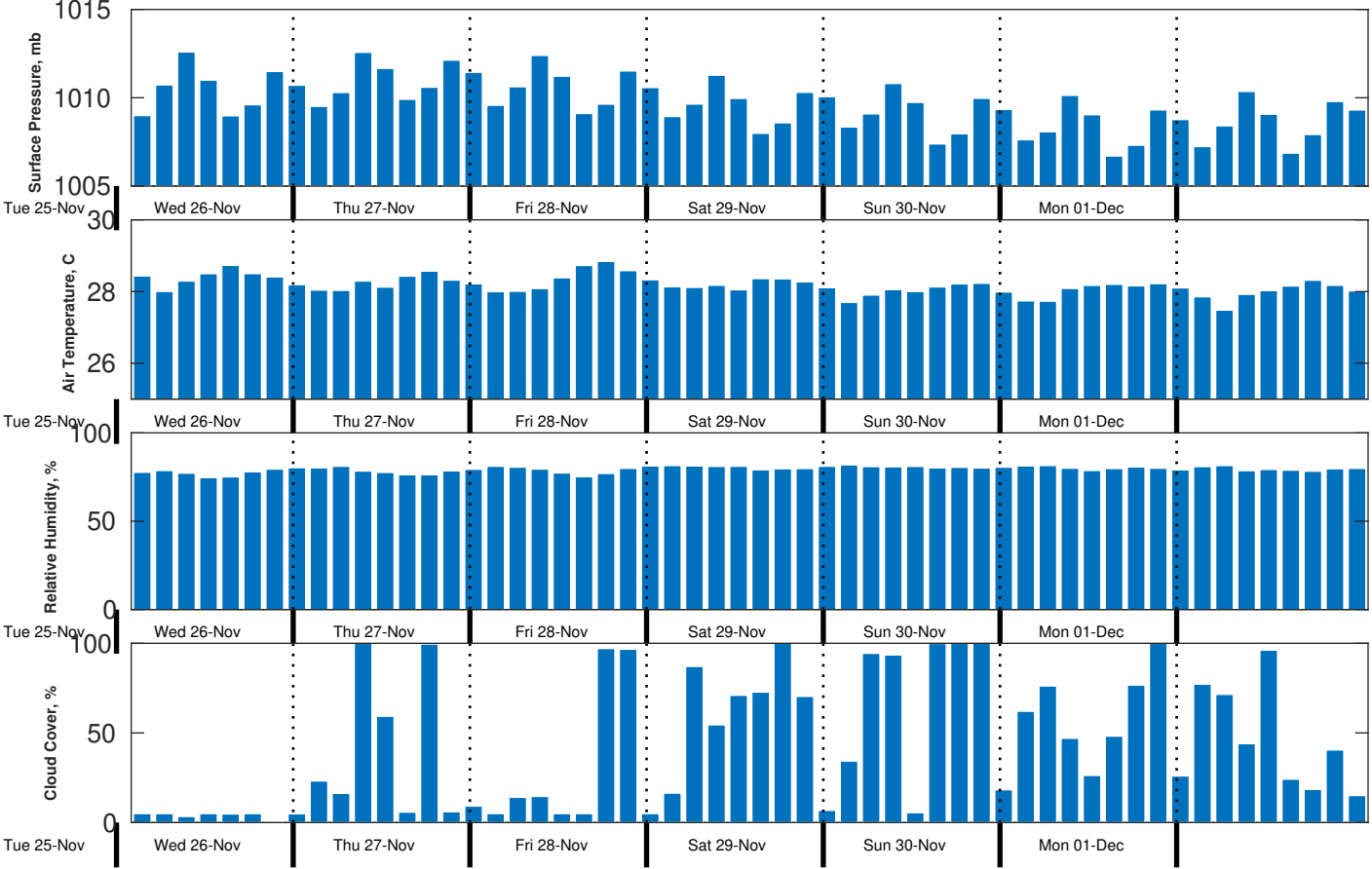
Met Forecast for CSA (ONHYM) PPL EBS - Cote d'Ivoire from 26-Nov-2025 00:00:00 to 03-Dec-2025 00:00:00
