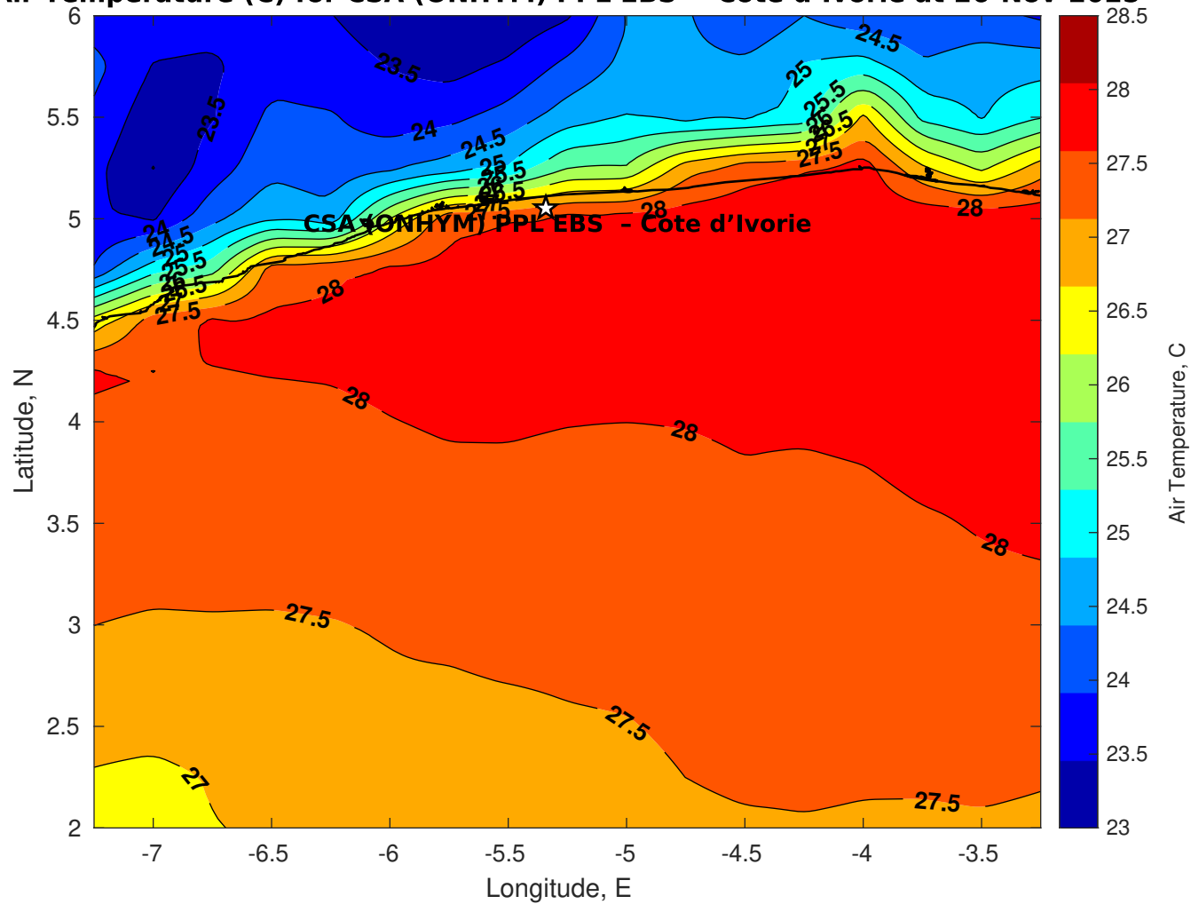
Air Temperature (C) for CSA (ONHYM) PPL EBS - Cote d'Ivoire at 26-Nov-2025
