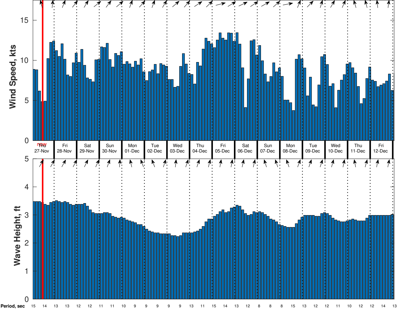
Wind & Wave Forecast for CSA (ONHYM) PPL EBS - Cote d'Ivoire from 26-Nov-2025 01:00:00 to 12-Dec-2025 01:00:00
