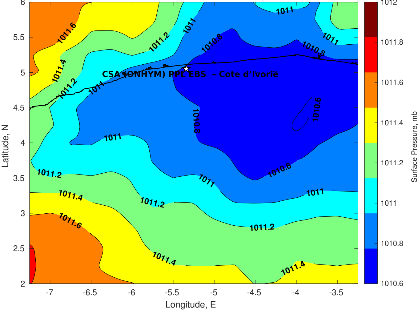
Surface Pressure (mb) for CSA (ONHYM) PPL EBS - Cote d'Ivoire at 27-Nov-2025 00:00:00
