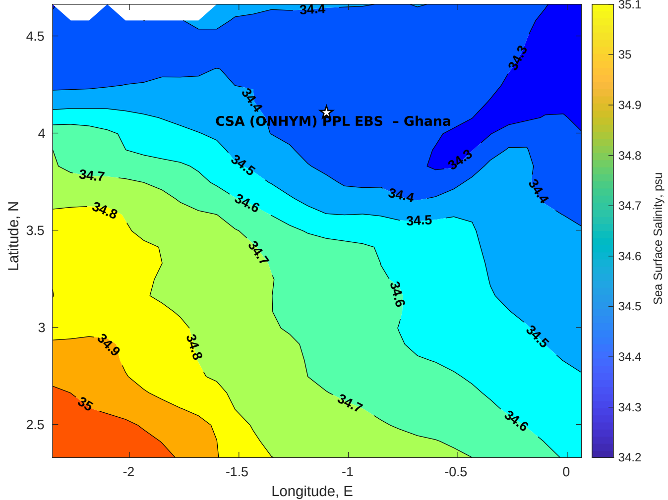
Surface Salinity for CSA (ONHYM) PPL EBS - Ghana at 25-Nov-2025 00:00:00
