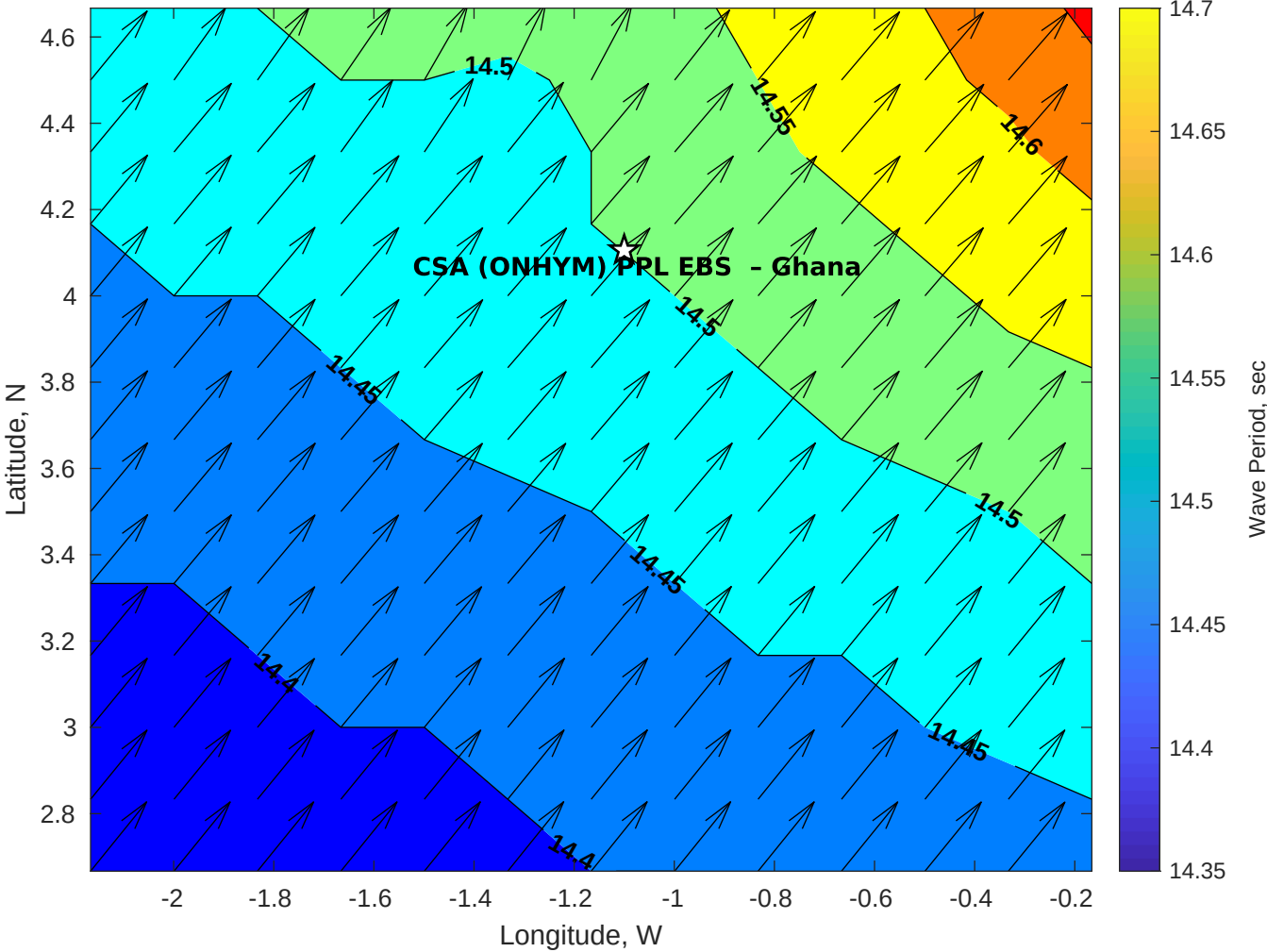
GFS Wave Period (sec) for CSA (ONHYM) PPL EBS - Ghana at 26-Nov-2025 09:00:00
