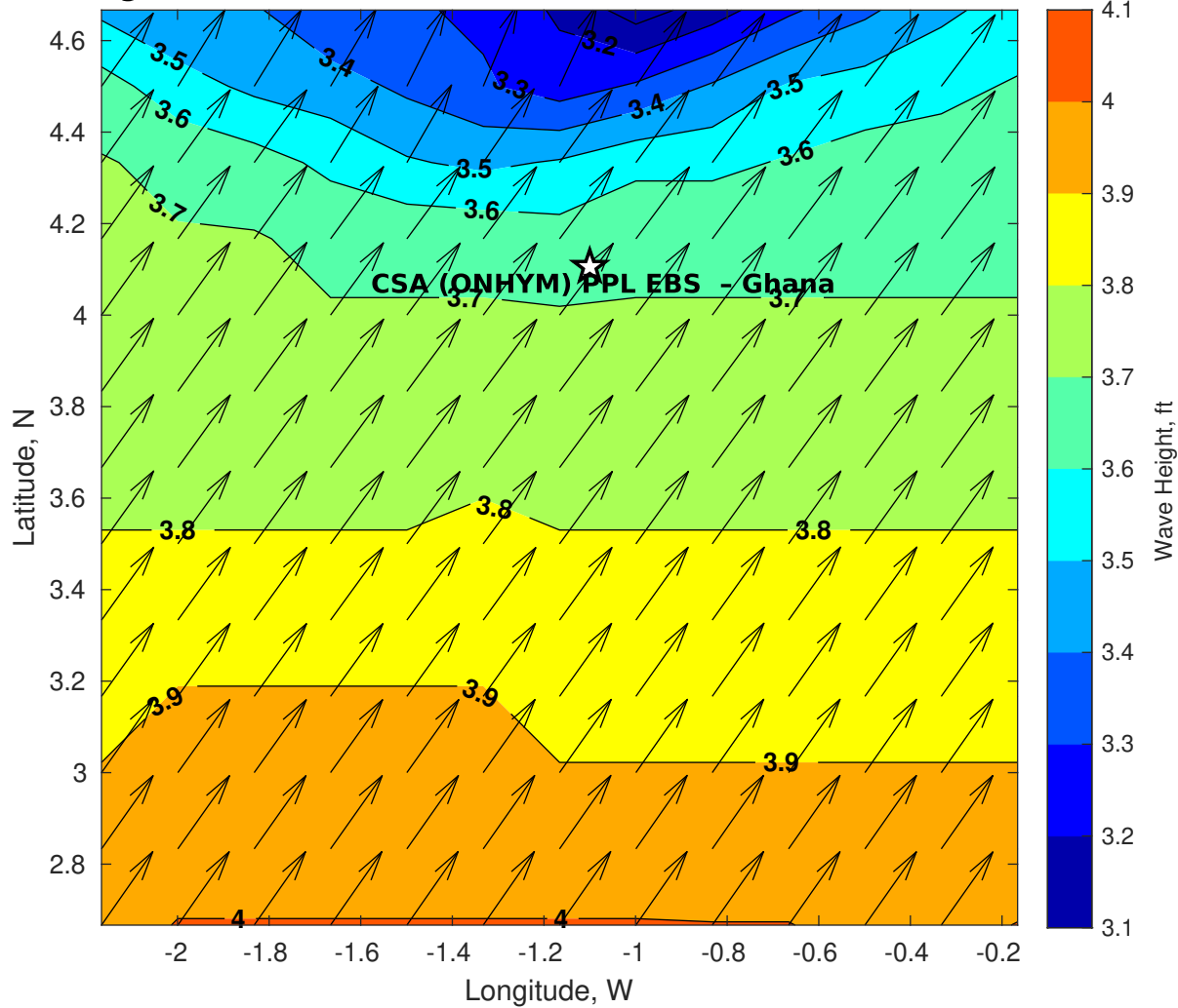
GFS Wave Height (ft) for CSA (ONHYM) PPL EBS - Ghana at 26-Nov-2025 09:00:00
