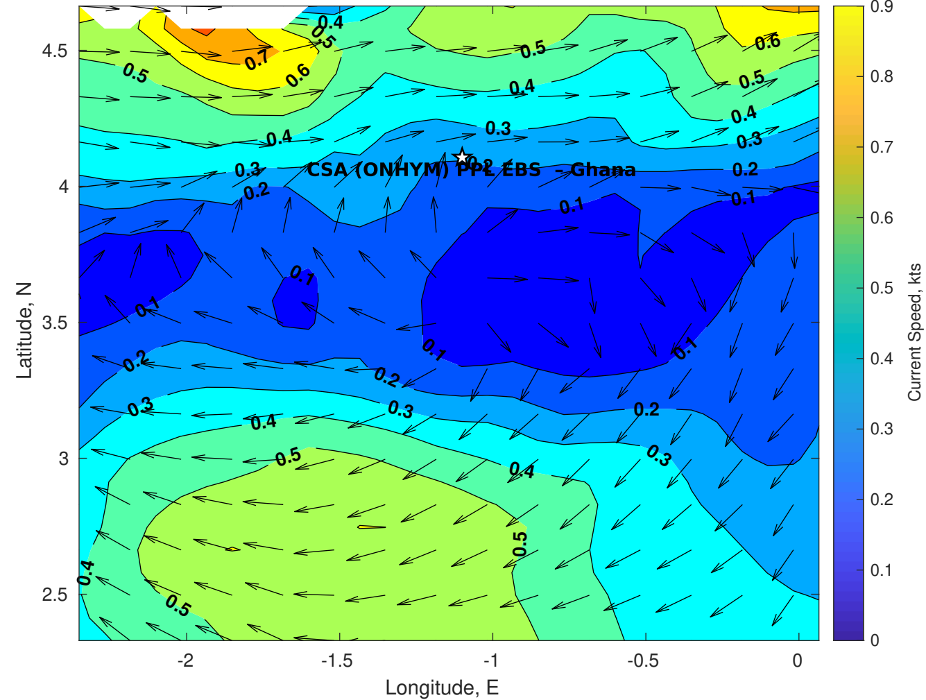
Surface Currents for CSA (ONHYM) PPL EBS - Ghana at 25-Nov-2025 00:00:00
