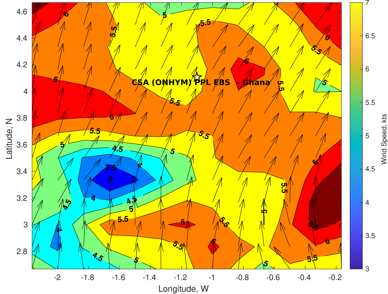
GFS Winds (kts) for CSA (ONHYM) PPL EBS - Ghana at 26-Nov-2025 09:00:00
