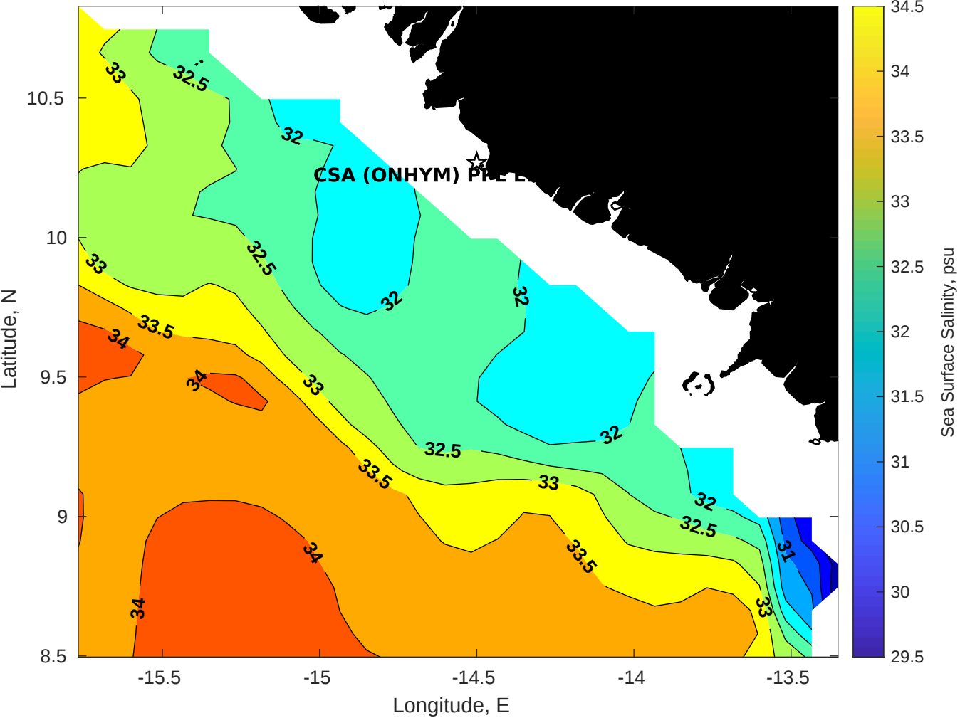
Surface Salinity for CSA (ONHYM) PPL EBS - Guinea at 25-Nov-2025 00:00:00
