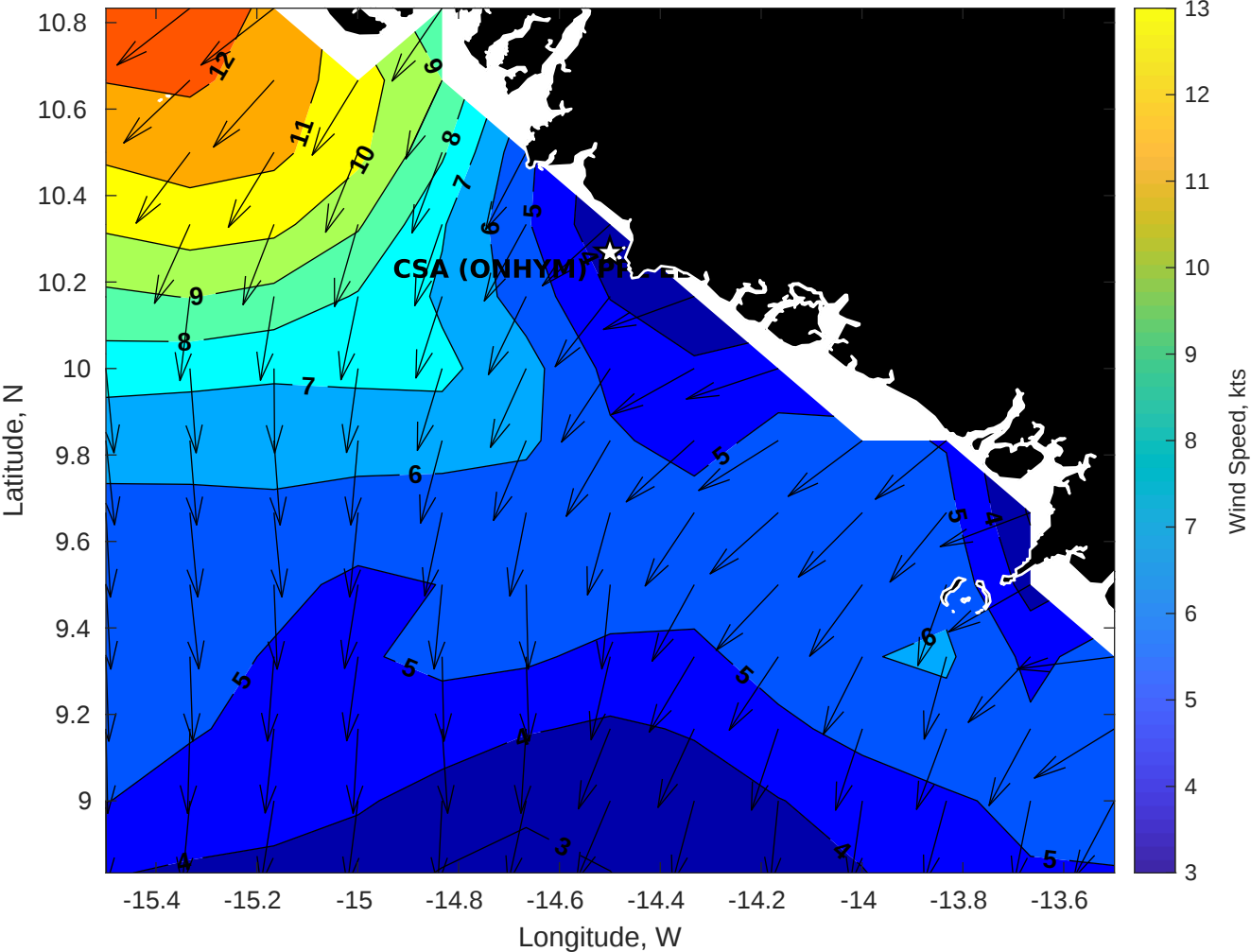
GFS Winds (kts) for CSA (ONHYM) PPL EBS - Guinea at 26-Nov-2025 09:00:00
