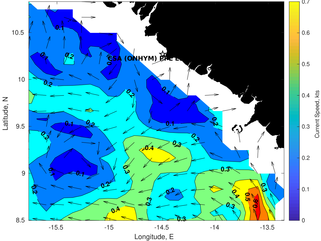
Surface Currents for CSA (ONHYM) PPL EBS - Guinea at 25-Nov-2025 00:00:00
