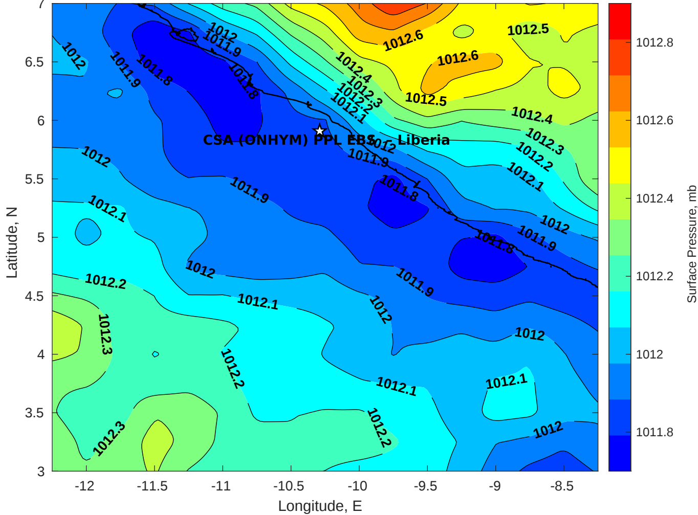
Surface Pressure (mb) for CSA (ONHYM) PPL EBS - Liberia at 28-Nov-2025 00:00:00
